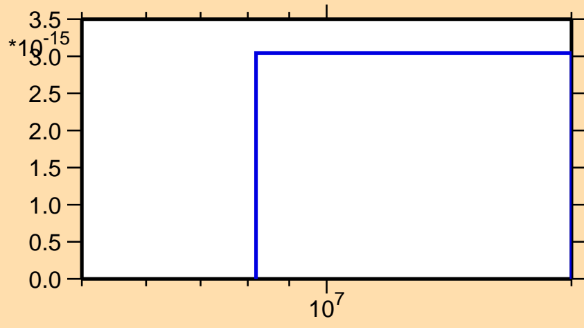
\sigma vs. E for ^{104}\text{Pd}(\text{mt117})
