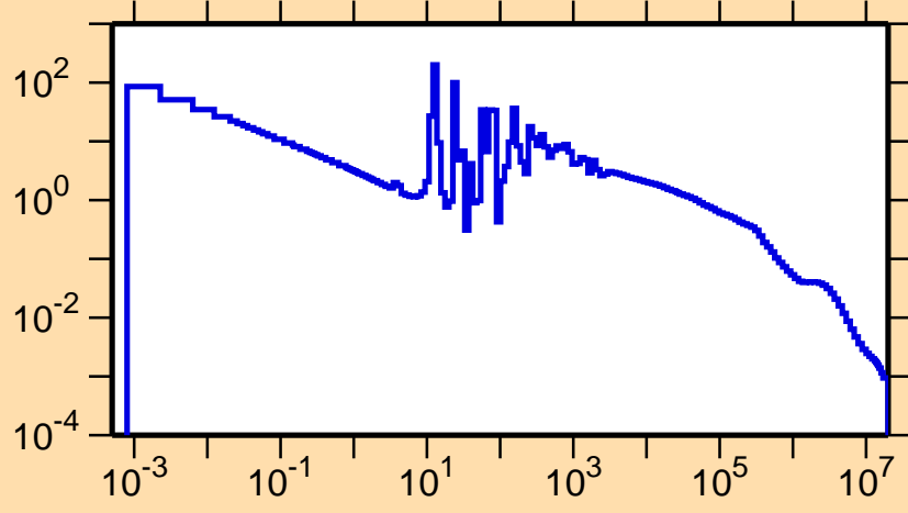
\sigma vs. E for ^{105}\text{Pd}(n,\gamma)
