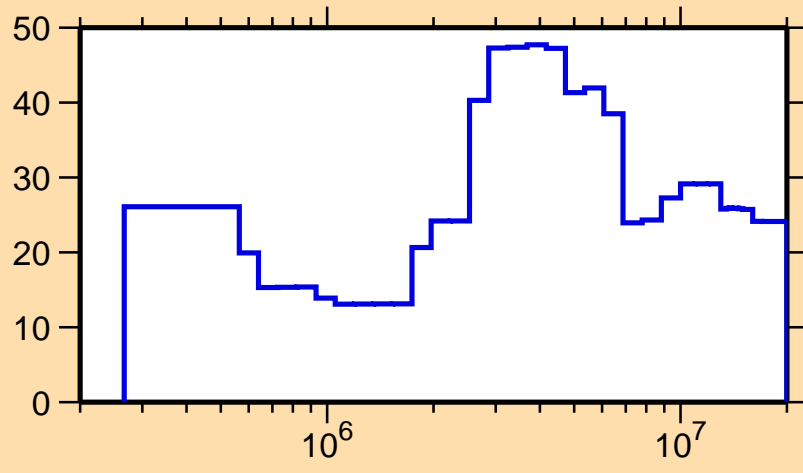
\Delta\sigma/\sigma vs. E for ^{105}\text{Pd}(n,n_1)
