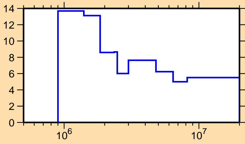
\Delta\sigma/\sigma vs. E for ^{105}\text{Pd}(n, tot.)
