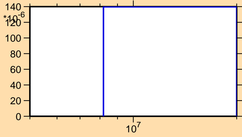
\sigma vs. E for ^{105}\text{Pd}(n,t)
