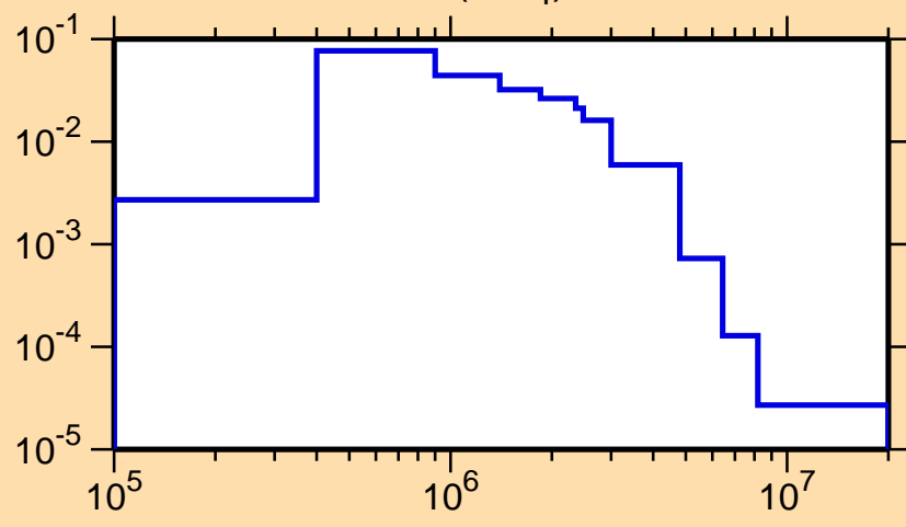
\sigma vs. E for ^{105}\text{Pd}(n,n_4)
