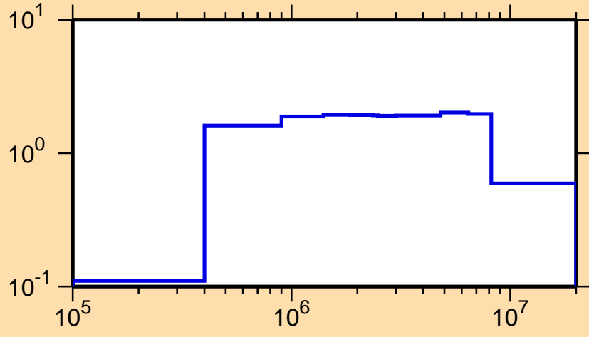
\sigma vs. E for ^{105}\text{Pd}(n,\text{inel.})
