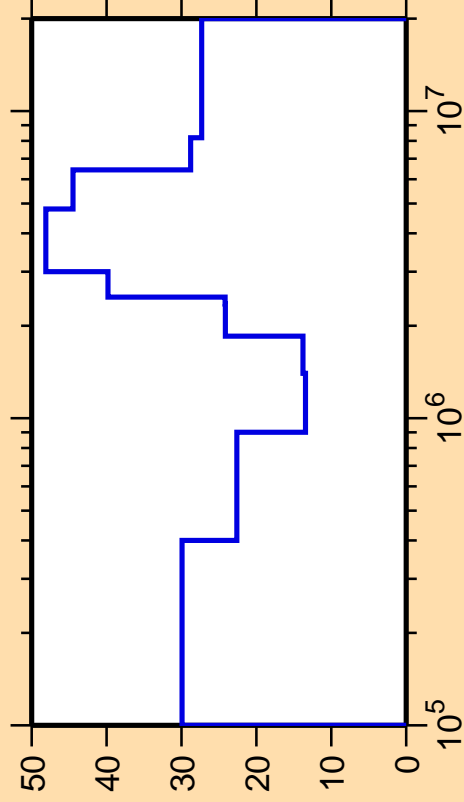
\Delta\sigma/\sigma vs. E for ^{105}\text{Pd}(n,n_4)
