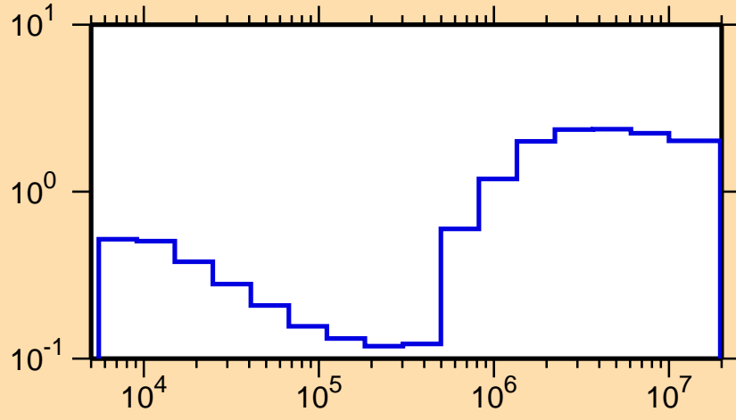
\sigma vs. E for ^{106}\text{Pd}(n,\text{nonel.})
