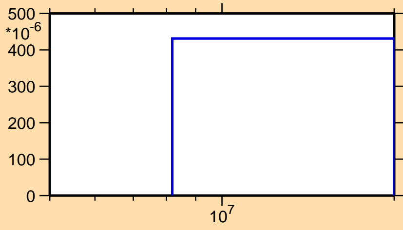
\sigma vs. E for ^{106}\text{Pd}(n,np)
