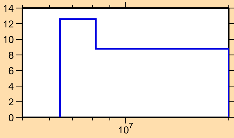
\Delta\sigma/\sigma vs. E for ^{107}\text{Pd}(n,2n)
