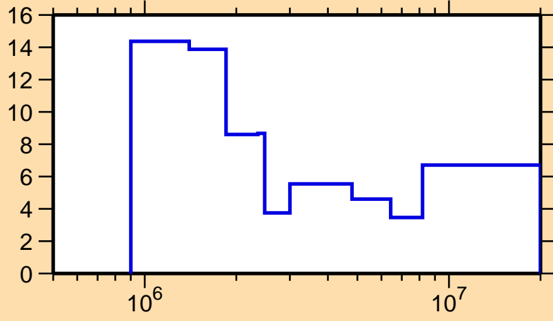
\Delta\sigma/\sigma vs. E for ^{107}\text{Pd}(n, tot.)
