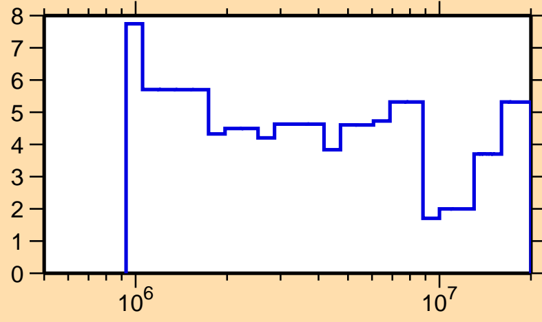
\Delta\sigma/\sigma vs. E for ^{107}\text{Pd}(n,\text{tot.})
