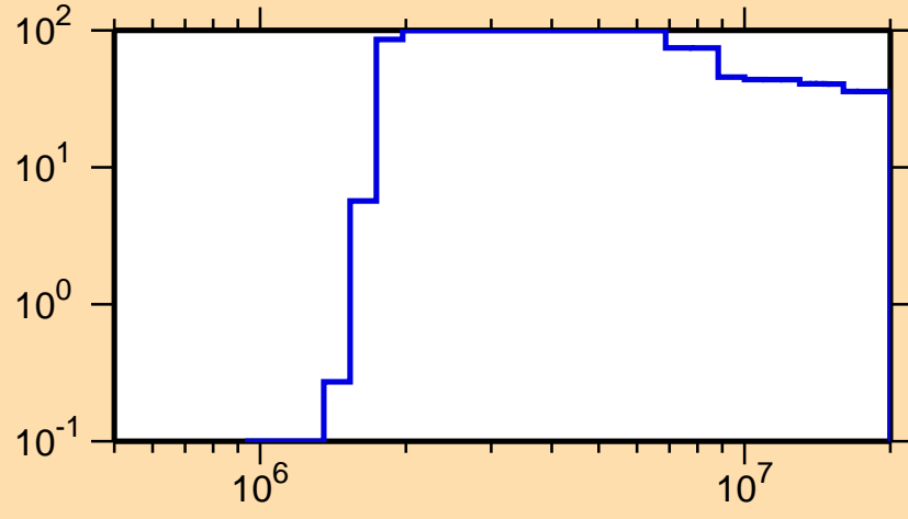
\Delta\sigma/\sigma vs. E for ^{107}\text{Pd}(n,p)
