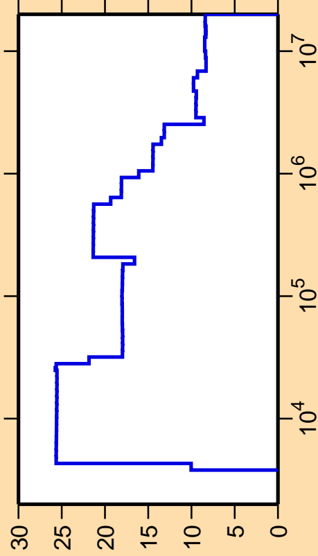
\Delta\sigma/\sigma vs. E for ^{107}\text{Pd}(n,\text{nonel.})
