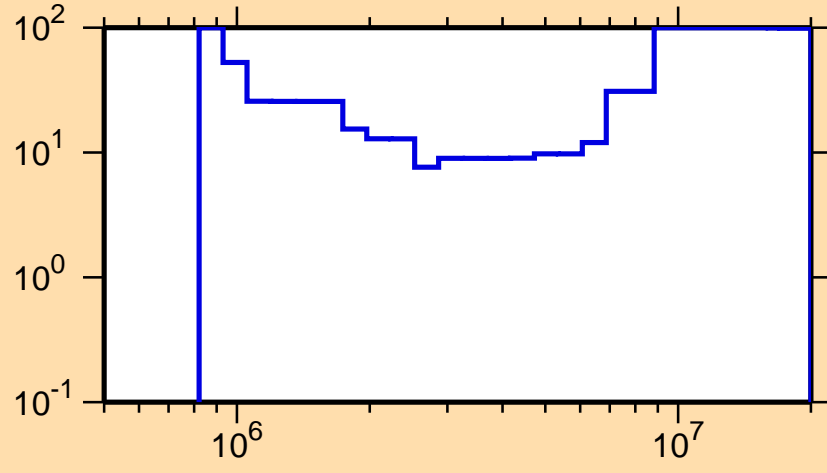
\Delta\sigma/\sigma vs. E for ^{107}\text{Pd}(n,n\text{cont.})
