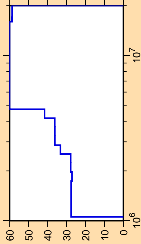
\Delta\sigma/\sigma vs. E for ^{108}\text{Pd}(n,n_3)
