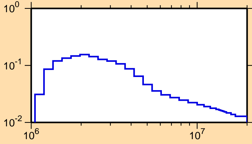
\sigma vs. E for ^{108}\text{Pd}(n,n_3)
