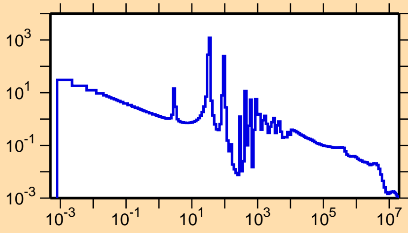
\sigma vs. E for ^{108}\text{Pd}(n,\gamma)
