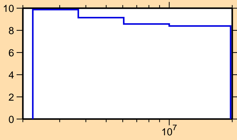
\Delta\sigma/\sigma vs. E for ^{108}\text{Pd}(n,n\text{onel.})
