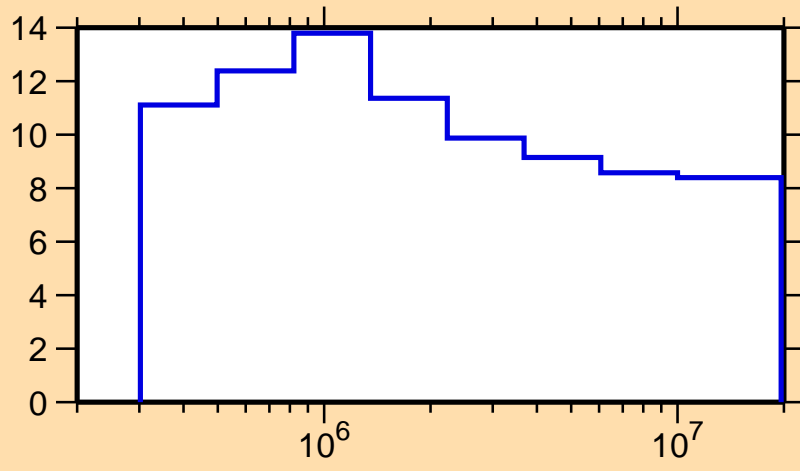
\Delta\sigma/\sigma vs. E for ^{108}\text{Pd}(n,\text{nonel.})
