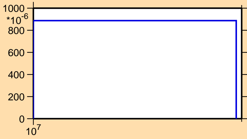
\sigma vs. E for ^{108}\text{Pd}(n,3n)
