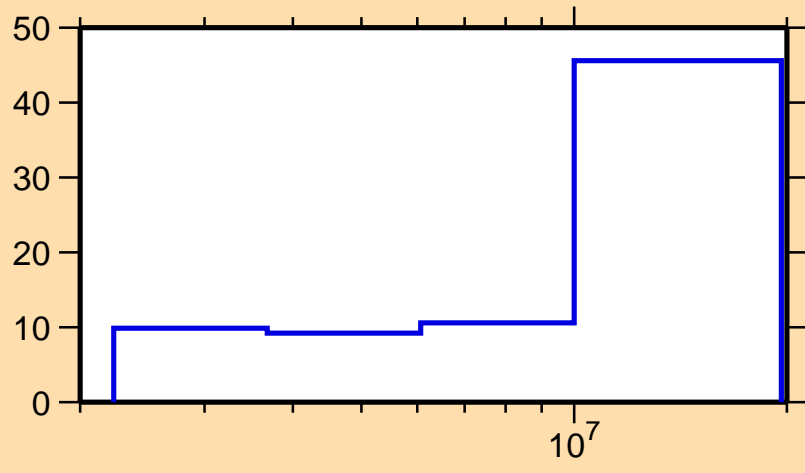
\Delta\sigma/\sigma vs. E for ^{108}\text{Pd}(n,\text{inel.})
