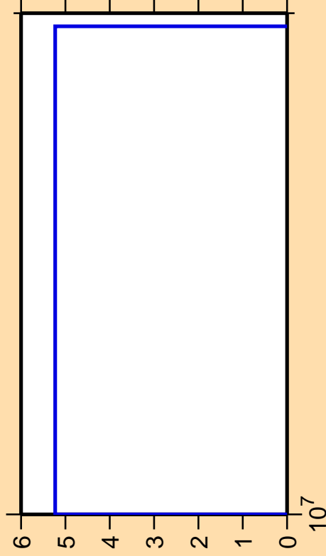
\Delta\sigma/\sigma vs. E for ^{108}\text{Pd}(n,\text{He}3)
