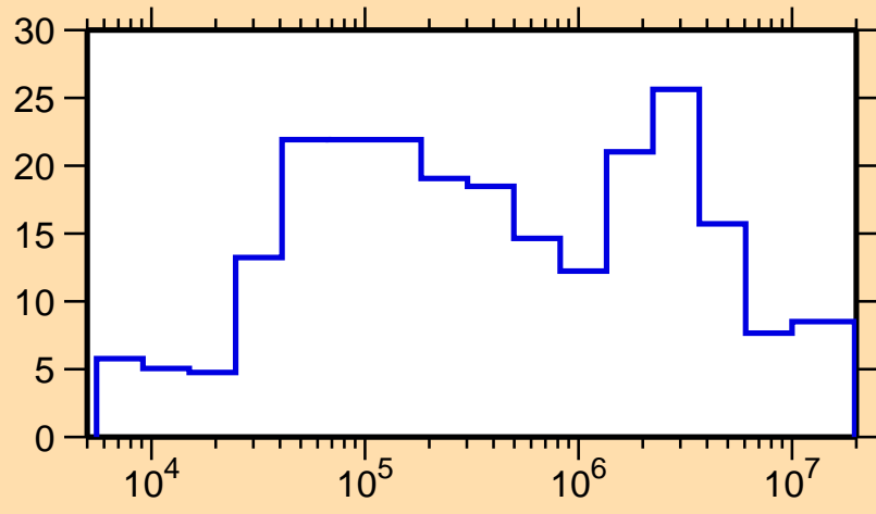
\Delta\sigma/\sigma vs. E for ^{108}\text{Pd}(n,\text{el.})
