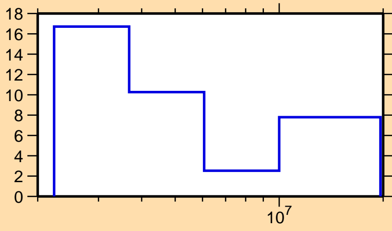
\Delta\sigma/\sigma vs. E for ^{108}\text{Pd}(n,\text{tot.})
