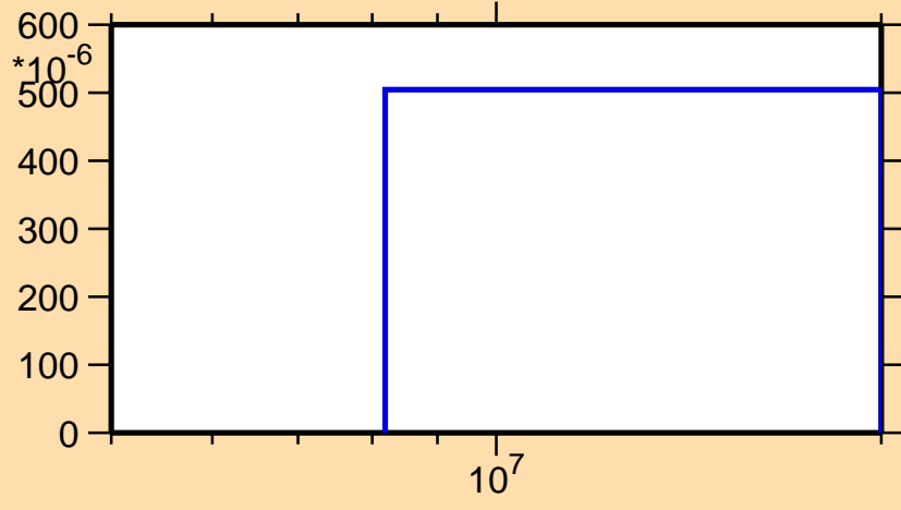
\sigma vs. E for ^{108}\text{Pd}(n,d)
