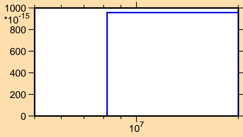
\sigma vs. E for ^{108}\text{Pd}(n,\text{He}3)
