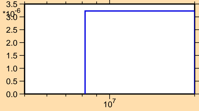
\sigma vs. E for ^{108}\text{Pd}(n,t)
