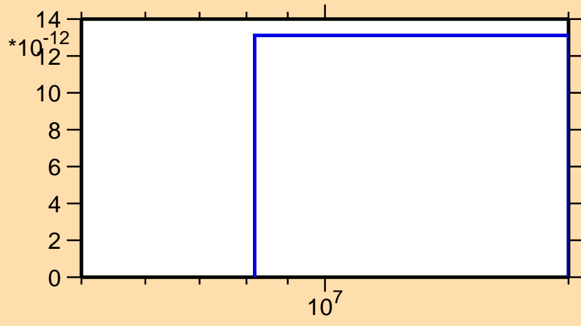
\sigma vs. E for ^{108}\text{Pd}(n,nd)
