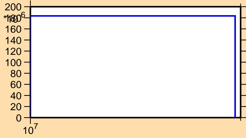
\sigma vs. E for ^{109}\text{Pd}(n,np)
