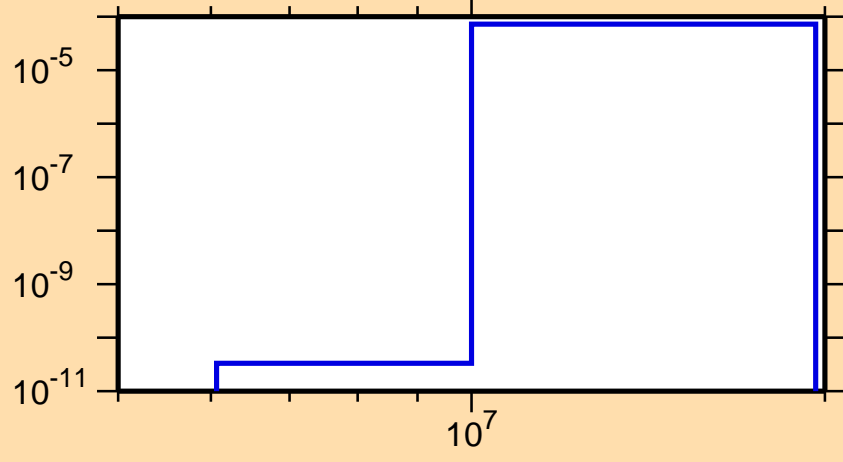
\sigma vs. E for ^{109}\text{Pd}(n,n\alpha)
