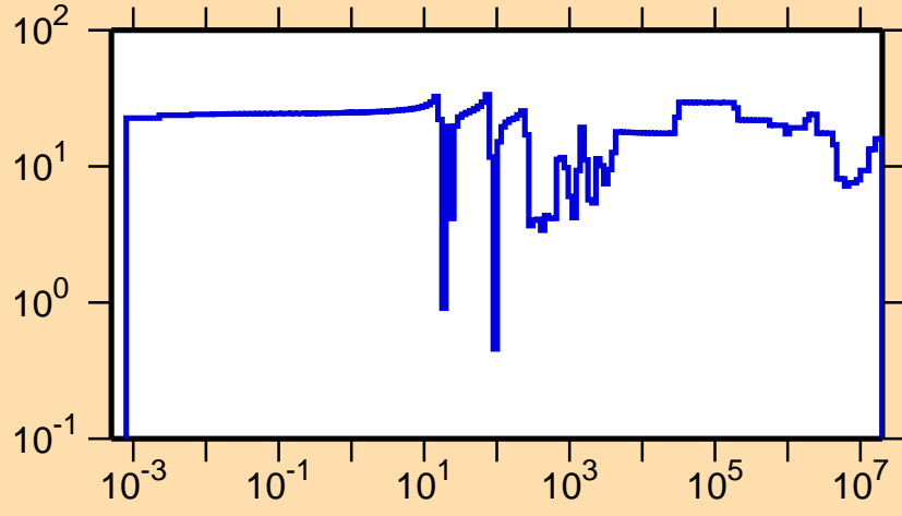
\Delta\sigma/\sigma vs. E for ^{109}\text{Pd}(n,\text{el.})
