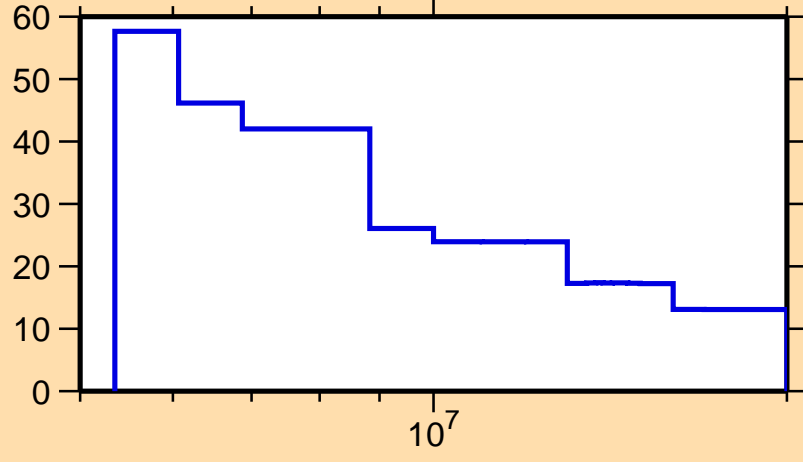
\Delta\sigma/\sigma vs. E for ^{109}\text{Pd}(n,2n)
