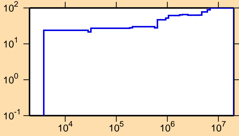
\Delta\sigma/\sigma vs. E for ^{109}\text{Pd}(n,n_1)
