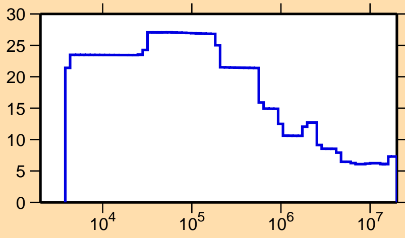
\Delta\sigma/\sigma vs. E for ^{109}\text{Pd}(n,\text{nonel.})
