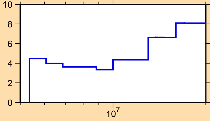
\Delta\sigma/\sigma vs. E for ^{109}\text{Pd}(n,\text{tot.})
