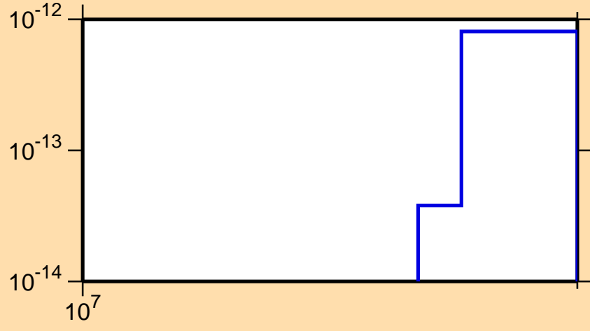
\sigma vs. E for ^{109}\text{Pd}(n,p\alpha)
