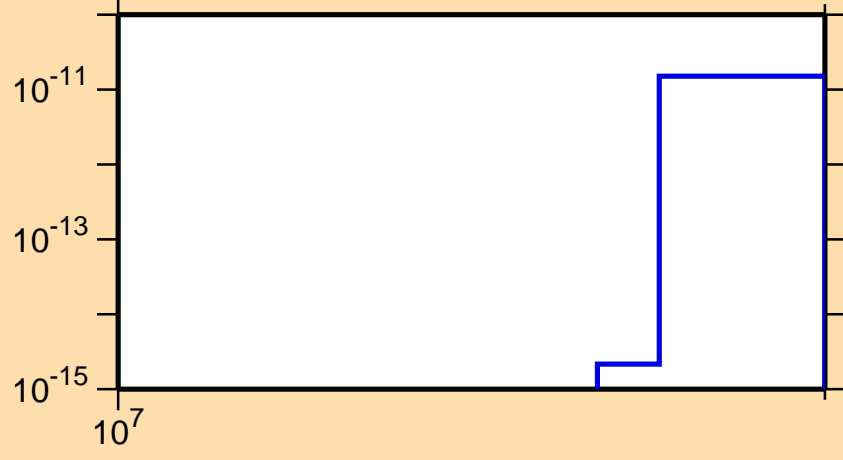
\sigma vs. E for ^{109}\text{Pd}(n,\text{He}3)
