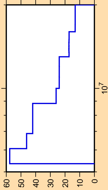
\Delta\sigma/\sigma vs. E for ^{109}\text{Pd}(n,2n)
