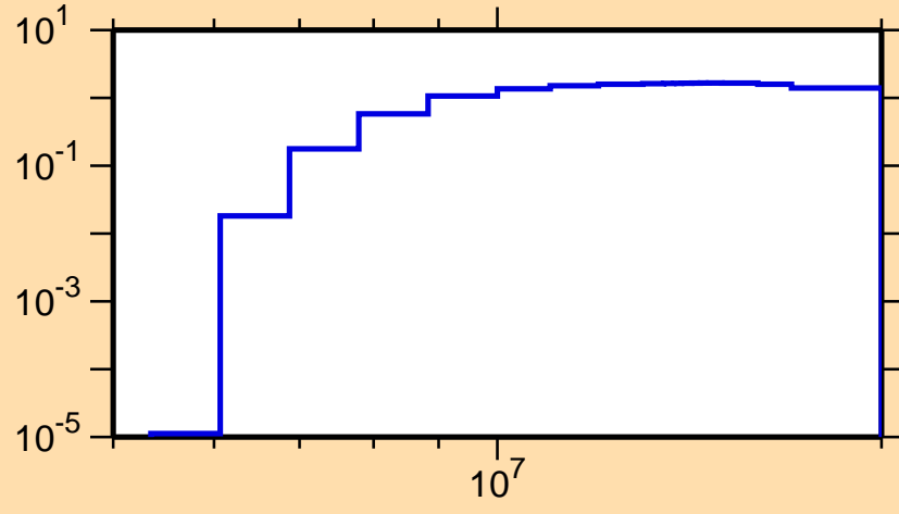
\sigma vs. E for ^{109}\text{Pd}(n,2n)
