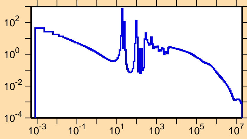
\sigma vs. E for ^{109}\text{Pd}(n,\gamma)
