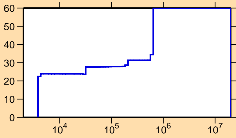
\Delta\sigma/\sigma vs. E for ^{109}\text{Pd}(n,\gamma)
