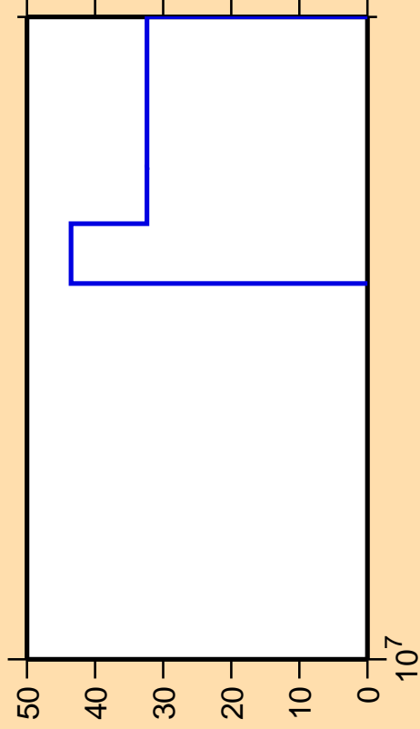
\Delta\sigma/\sigma vs. E for ^{109}\text{Pd}(n,3n)
