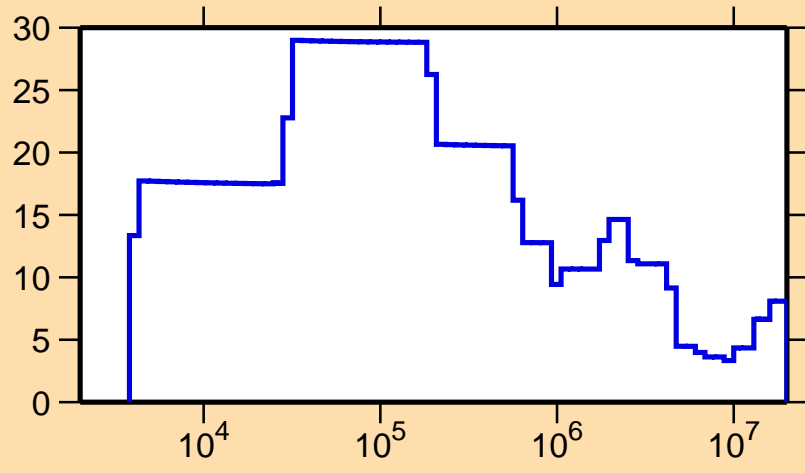
\Delta\sigma/\sigma vs. E for ^{109}\text{Pd}(n,\text{tot.})
