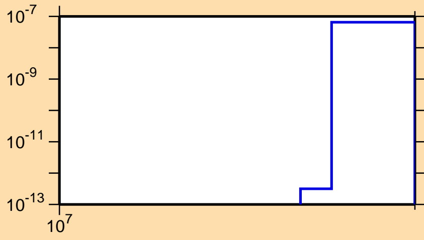
\sigma vs. E for ^{109}\text{Pd}(n,2np)
