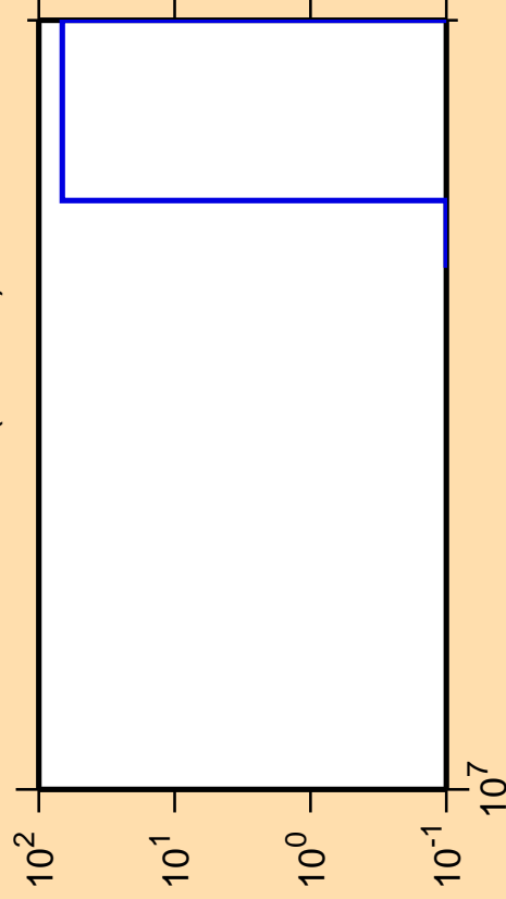
\Delta\sigma/\sigma vs. E for ^{109}\text{Pd}(n,\text{He}3)
