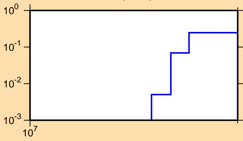
\sigma vs. E for ^{109}\text{Pd}(n,3n)
