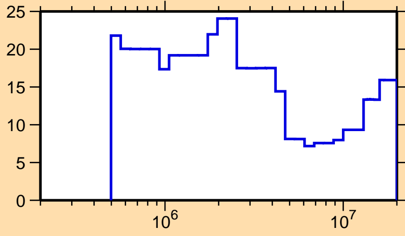
\Delta\sigma/\sigma vs. E for ^{109}\text{Pd}(n,\text{el.})
