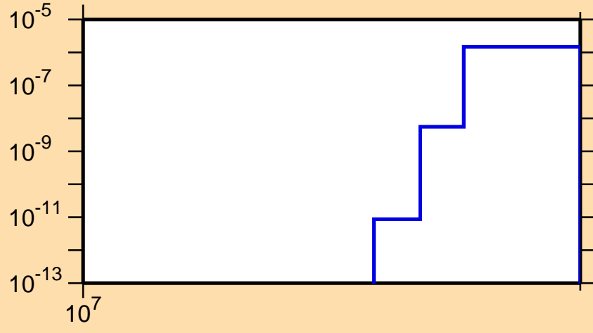
\sigma vs. E for ^{109}\text{Pd}(n,\text{nd})
