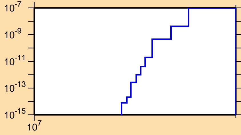
\sigma vs. E for ^{109}\text{Pd}(n,2n\alpha)
