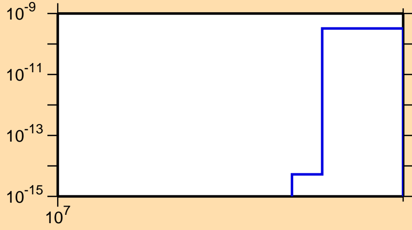
\sigma vs. E for ^{109}\text{Pd}(n,nt)
