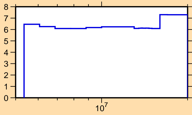
\Delta\sigma/\sigma vs. E for ^{109}\text{Pd}(n,\text{nonel.})
