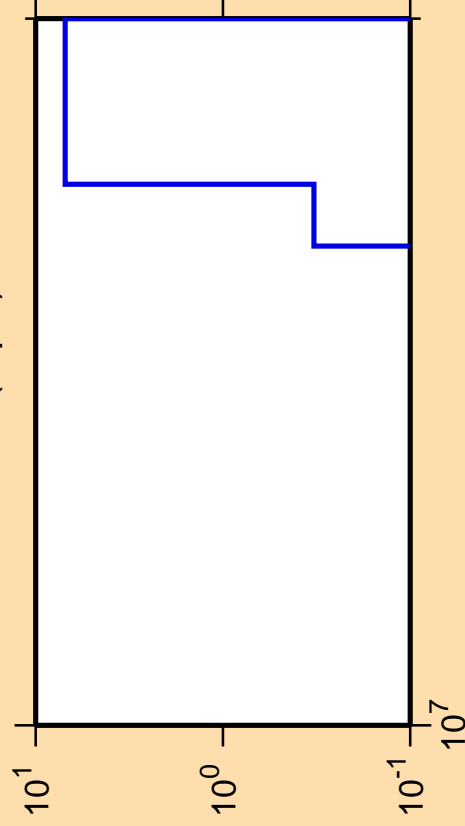
\Delta\sigma/\sigma vs. E for ^{109}\text{Pd}(n,p\alpha)
