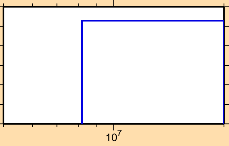
\sigma vs. E for ^{109}\text{Pd}(n,3n)
