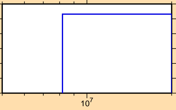
\sigma vs. E for ^{109}\text{Pd}(n,2np)
