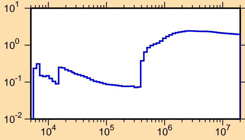
\sigma vs. E for ^{110}\text{Pd}(n,\text{nonel.})
