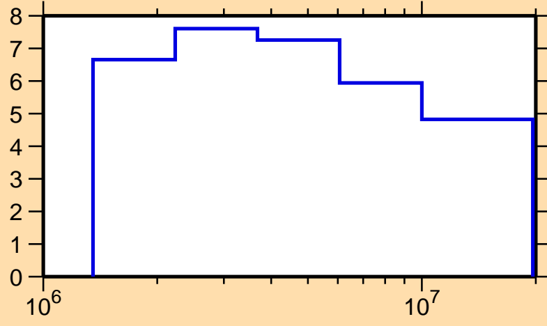
\Delta\sigma/\sigma vs. E for ^{110}\text{Pd}(n,n\text{onel.})
