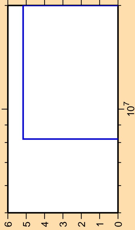
\Delta\sigma/\sigma vs. E for ^{110}\text{Pd}(n,nd)
