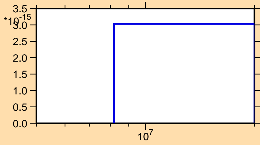
\sigma vs. E for ^{110}\text{Pd}(n,\text{He3})
