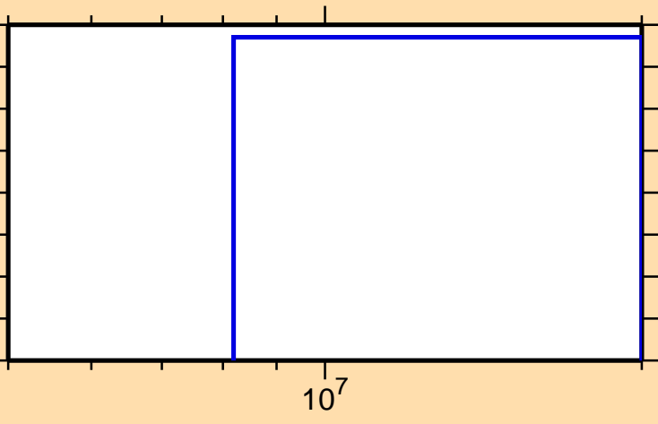
\sigma vs. E for ^{110}\text{Pd}(n,np)
