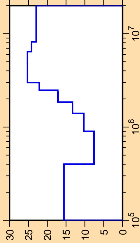
\Delta\sigma/\sigma vs. E for ^{110}\text{Pd}(n,n_1)
