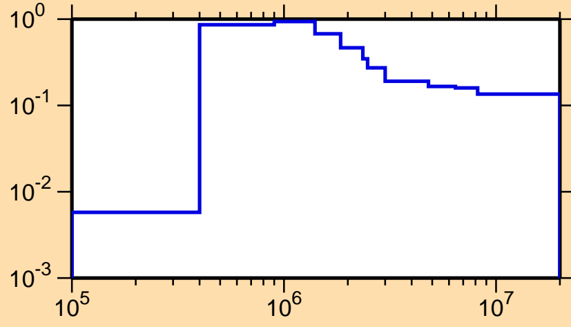
\sigma vs. E for ^{110}\text{Pd}(n,n_1)
