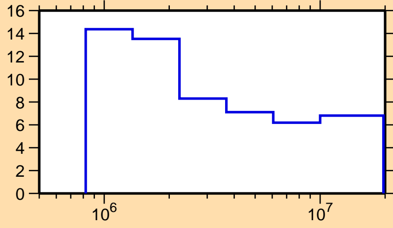
\Delta\sigma/\sigma vs. E for ^{111}\text{Pd}(n,n\text{onel.})
