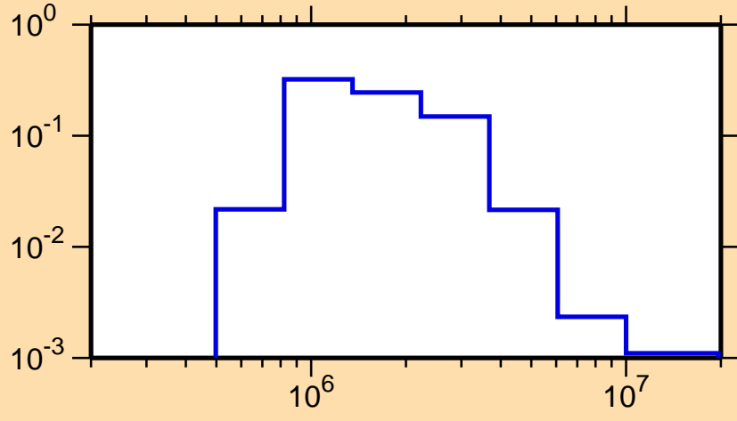
\sigma vs. E for ^{112}\text{Pd}(n,n_2)
