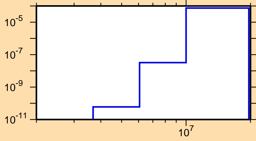
\sigma vs. E for ^{112}\text{Pd}(n,\alpha)
