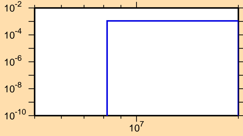
\sigma vs. E for ^{112}\text{Pd}(n,p)
