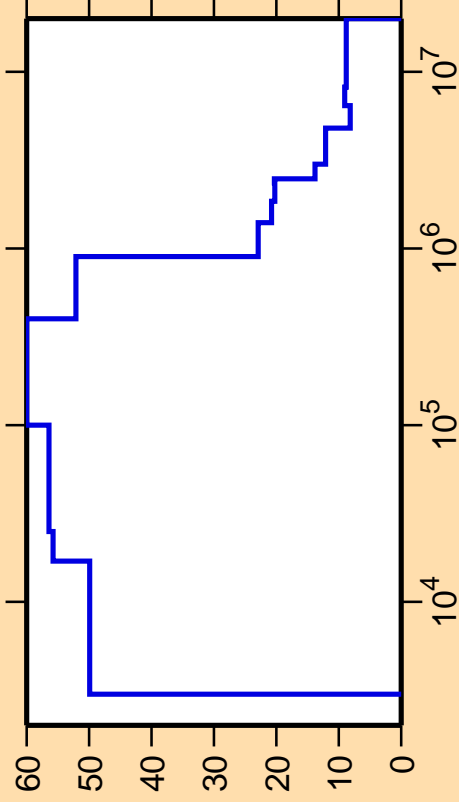
\Delta\sigma/\sigma vs. E for ^{112}\text{Pd}(n,\text{nonel.})
