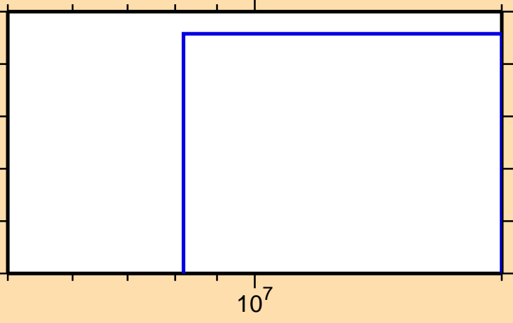
\sigma vs. E for ^{112}\text{Pd}(n,2n\alpha)
