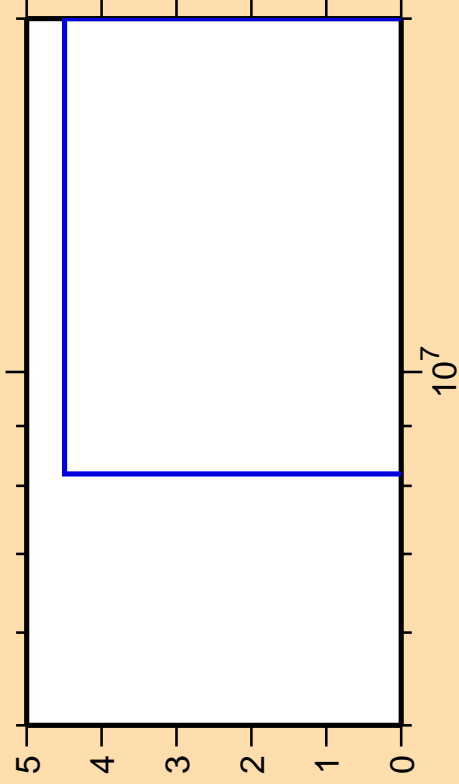
\Delta\sigma/\sigma vs. E for ^{112}\text{Pd}(n,nt)
