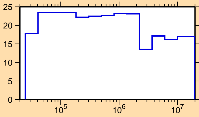
\Delta\sigma/\sigma vs. E for ^{113}\text{Pd}(n,\text{el.})
