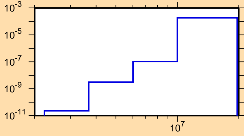
\sigma vs. E for ^{113}\text{Pd}(n,\alpha)
