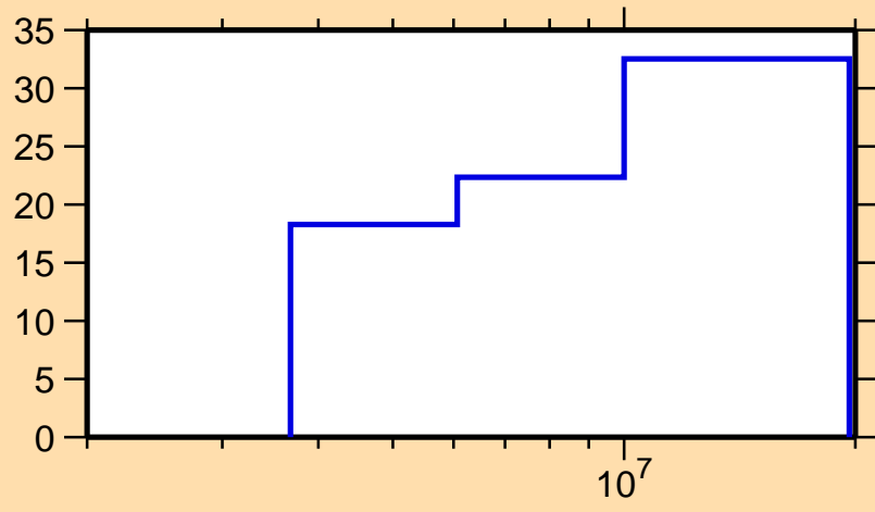
\Delta\sigma/\sigma vs. E for ^{113}\text{Pd}(n,2n)
