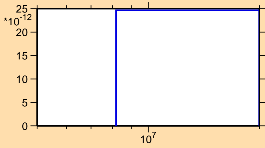
\sigma vs. E for ^{113}\text{Pd}(n,2np)
