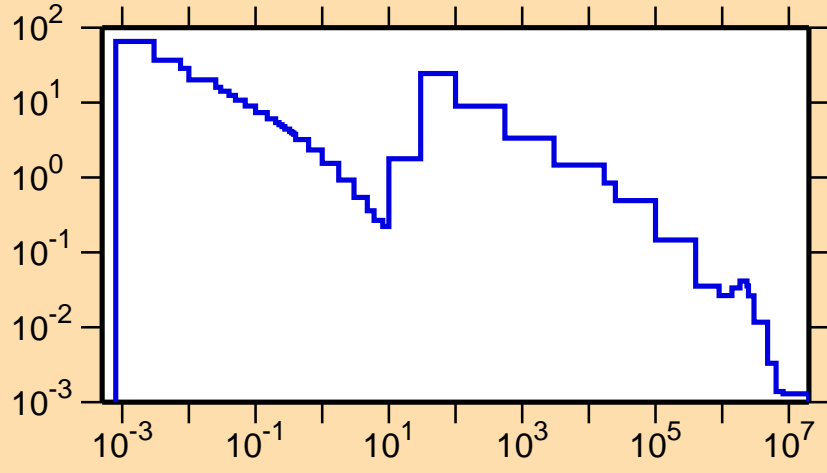
\sigma vs. E for ^{113}\text{Pd}(n,\gamma)
