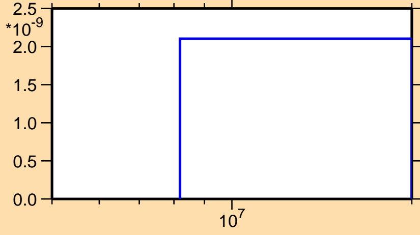
\sigma vs. E for ^{113}\text{Pd}(n,\text{nd})
