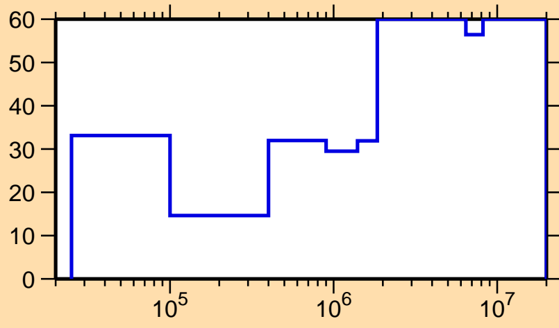
\Delta\sigma/\sigma vs. E for ^{113}\text{Pd}(n,n_1)
