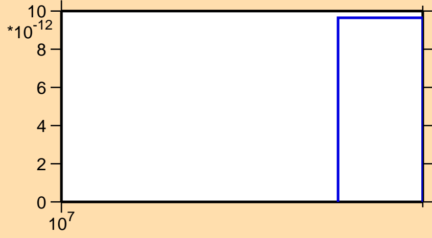
\sigma vs. E for ^{114}\text{Pd}(n,nd)
