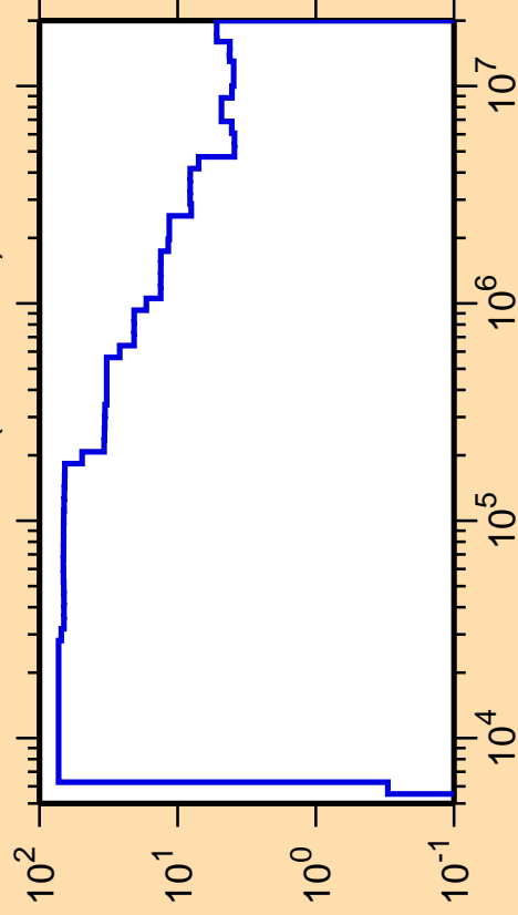
\Delta\sigma/\sigma vs. E for ^{114}\text{Pd}(n,\text{nonel.})
