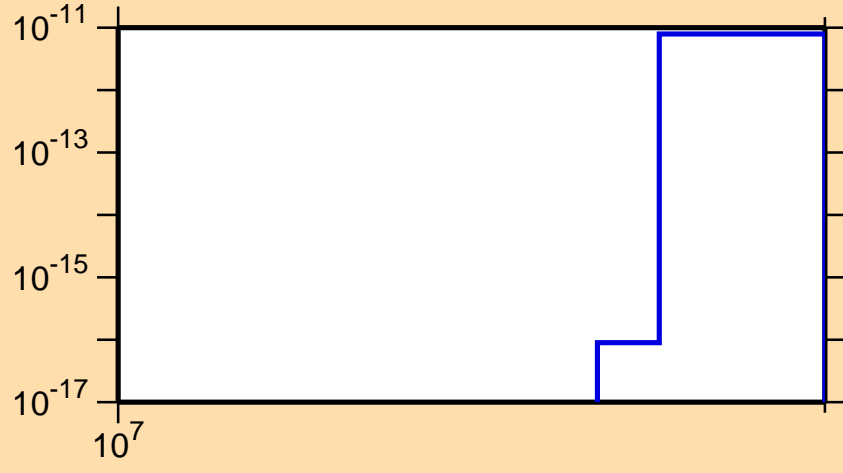
\sigma vs. E for ^{114}\text{Pd}(n,2n\alpha)
