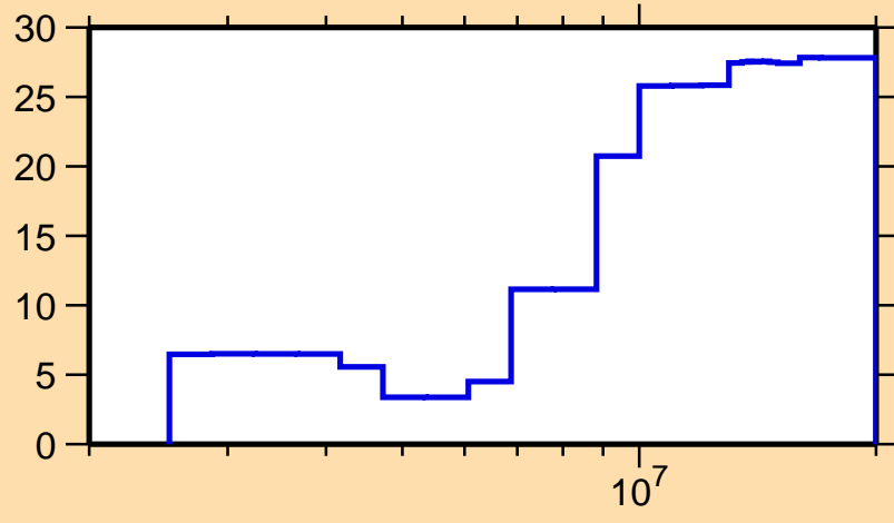
\Delta\sigma/\sigma vs. E for ^{114}\text{Pd}(n,\text{inel.})
