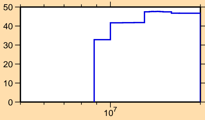
\Delta\sigma/\sigma vs. E for ^{114}\text{Pd}(n,n\text{cont.})
