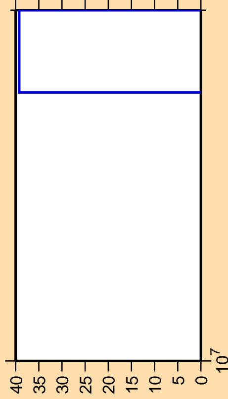
\Delta\sigma/\sigma vs. E for ^{114}\text{Pd}(n,nd)
