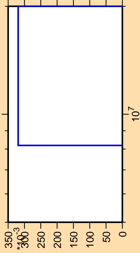
\Delta\sigma/\sigma vs. E for ^{114}\text{Pd}(n,nd)
