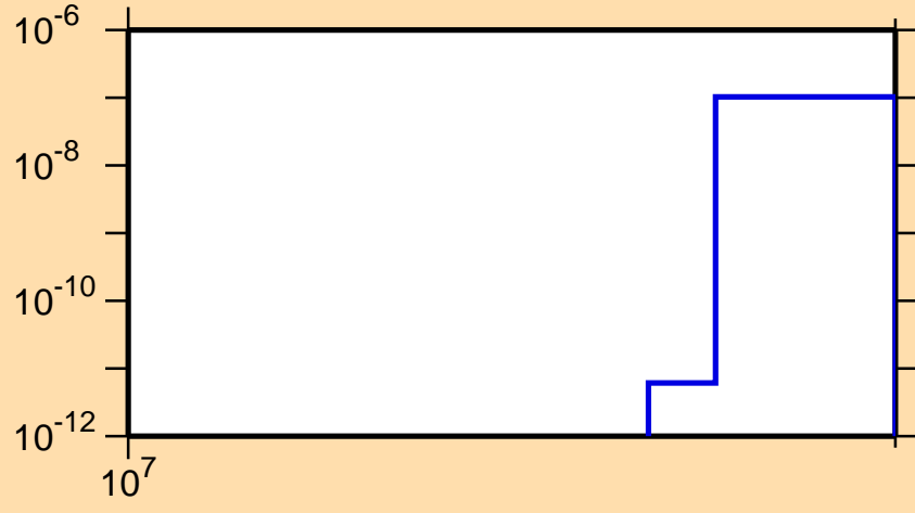
\sigma vs. E for ^{115}\text{Pd}(n,\text{nd})
