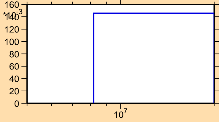
\sigma vs. E for ^{115}\text{Pd}(n,3n)
