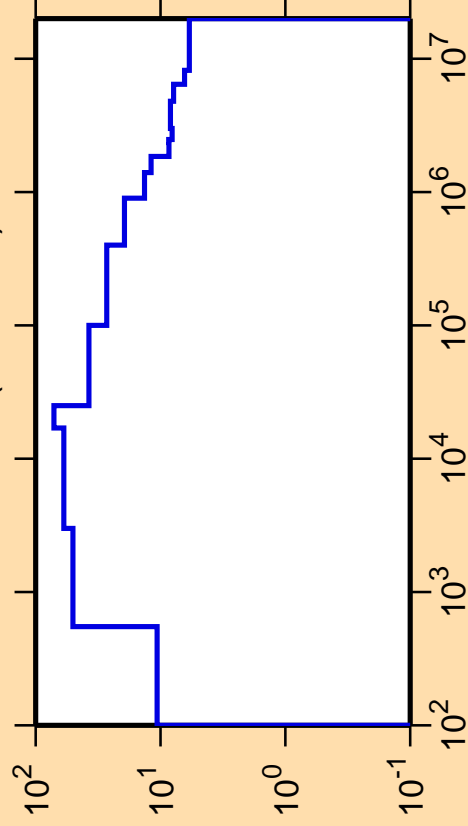
\Delta\sigma/\sigma vs. E for ^{115}\text{Pd}(n,\text{nonel.})
