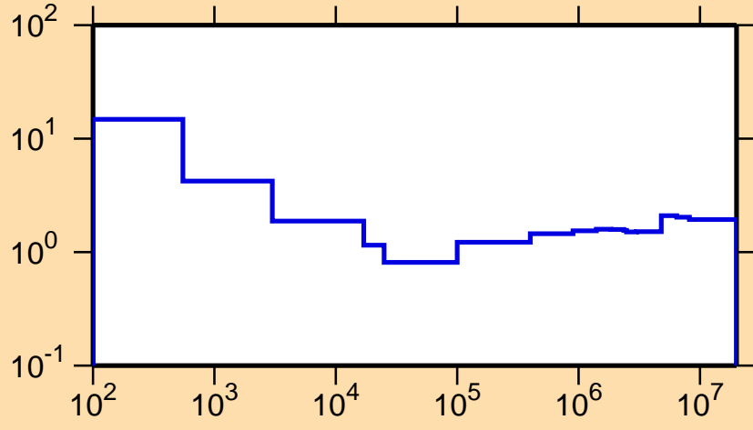
\sigma vs. E for ^{115}\text{Pd}(n,\text{nonel.})
