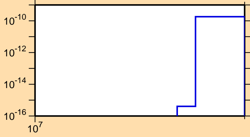
\sigma vs. E for ^{116}\text{Pd}(n,nt)
