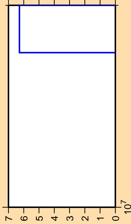
\Delta\sigma/\sigma vs. E for ^{116}\text{Pd}(n,\text{nd})
