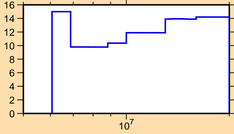
\Delta\sigma/\sigma vs. E for ^{116}\text{Pd}(n,\text{tot.})
