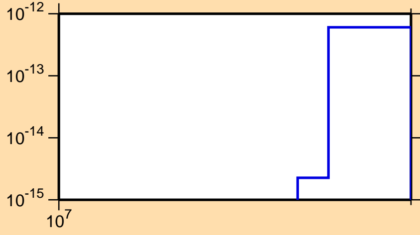
\sigma vs. E for ^{116}\text{Pd}(n,2n\alpha)
