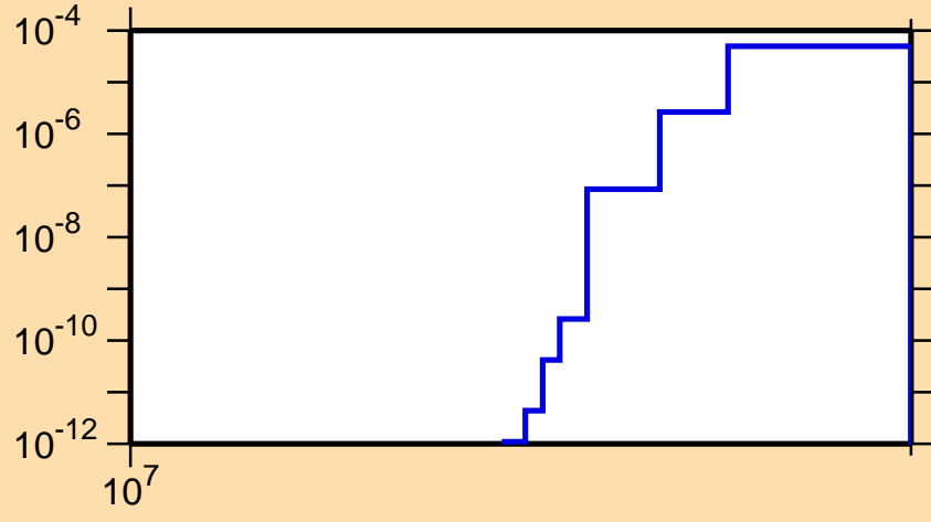
\sigma vs. E for ^{116}\text{Pd}(n,np)
