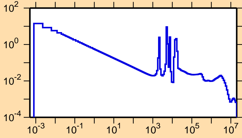
\sigma vs. E for ^{116}\text{Pd}(n,\gamma)
