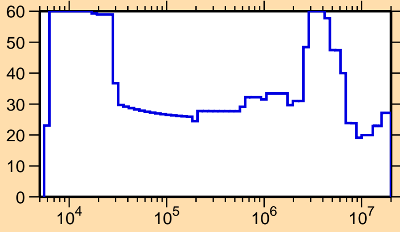
\Delta\sigma/\sigma vs. E for ^{116}\text{Pd}(n,\text{el.})
