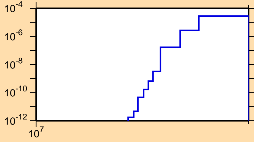
\sigma vs. E for ^{116}\text{Pd}(n,t)
