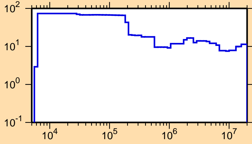
\Delta\sigma/\sigma vs. E for ^{116}\text{Pd}(n,\text{nonel.})
