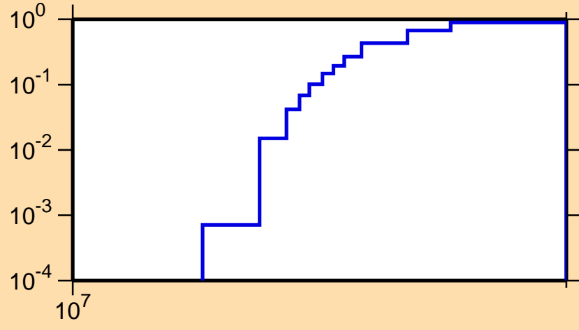
\sigma vs. E for ^{116}\text{Pd}(n,3n)
