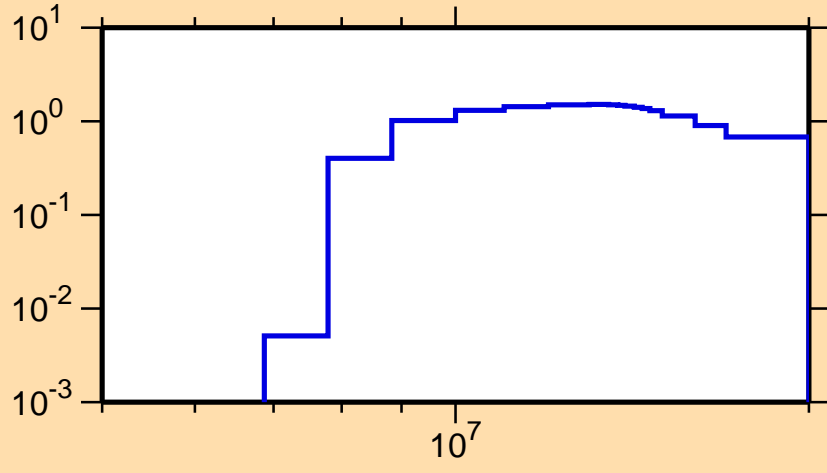
\sigma vs. E for ^{116}\text{Pd}(n,2n)
