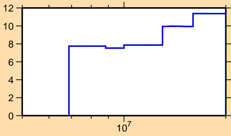
\Delta\sigma/\sigma vs. E for ^{116}\text{Pd}(n,\text{nonel.})
