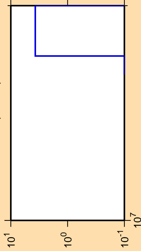
\Delta\sigma/\sigma vs. E for ^{116}\text{Pd}(n,2n\alpha)
