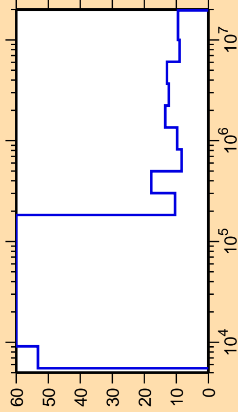
\Delta\sigma/\sigma vs. E for ^{116}\text{Pd}(n,\text{nonel.})
