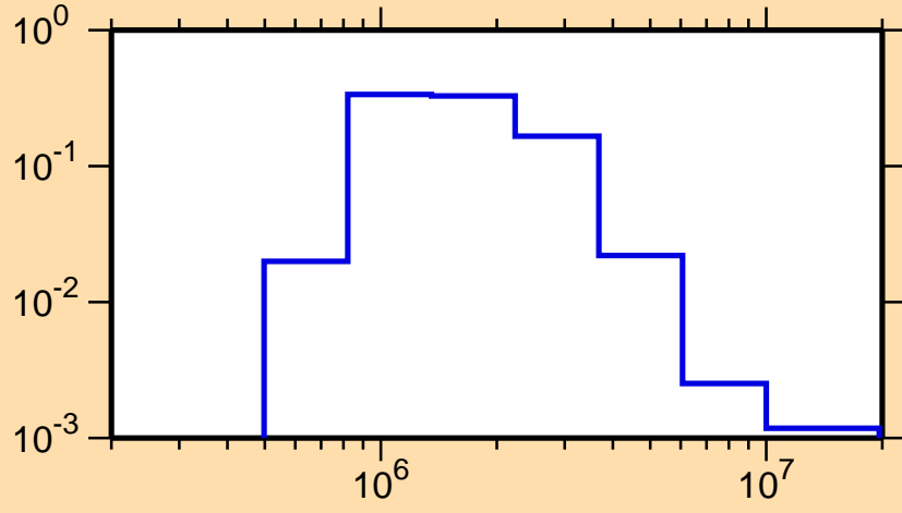
\sigma vs. E for ^{116}\text{Pd}(n,n_2)
