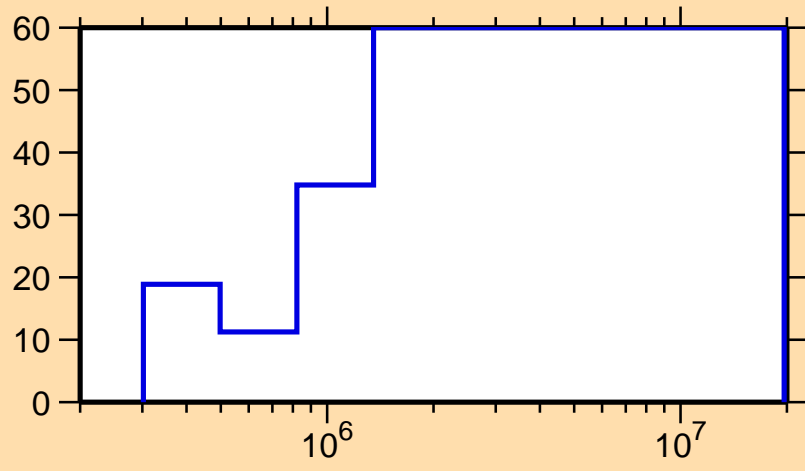
\Delta\sigma/\sigma vs. E for ^{116}\text{Pd}(n,n_1)
