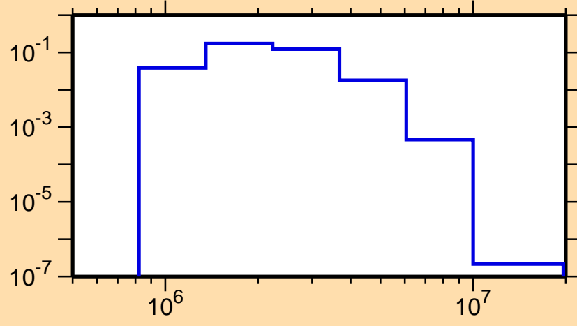
\sigma vs. E for ^{116}\text{Pd}(n,n_4)
