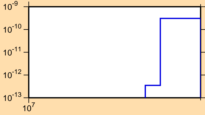
\sigma vs. E for ^{117}\text{Pd}(n,2n\alpha)
