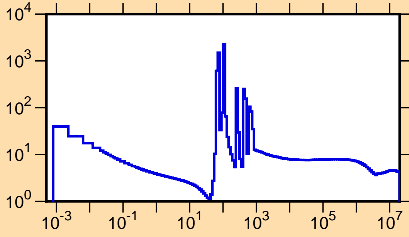
\sigma vs. E for ^{117}\text{Pd}(n,\text{tot.})
