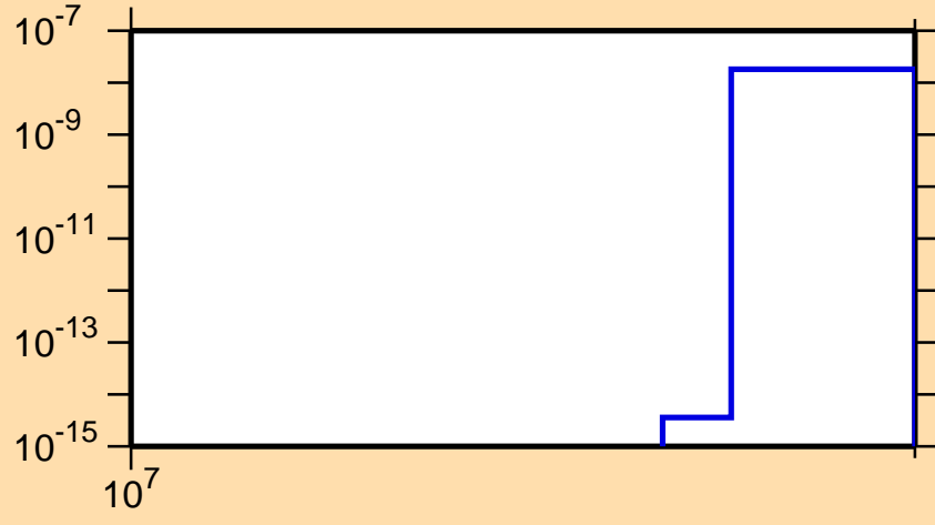
\sigma vs. E for ^{117}\text{Pd}(n,\text{nd})
