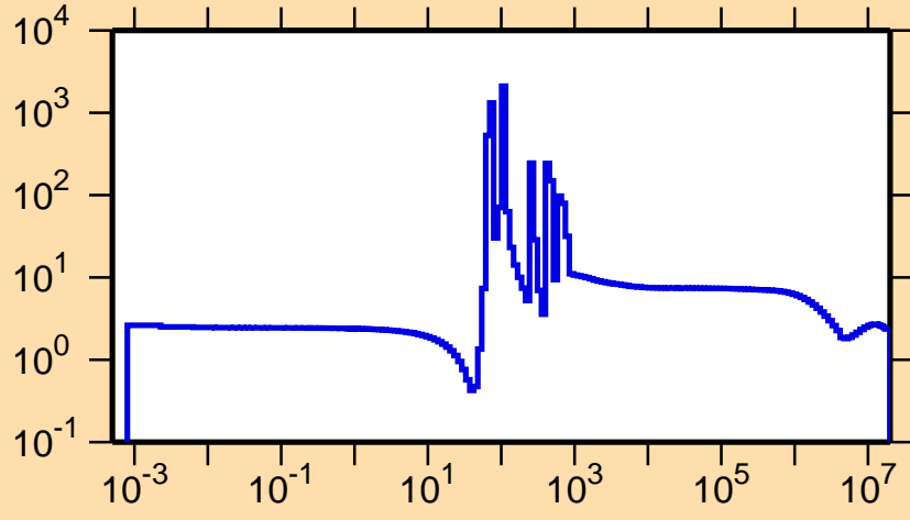
\sigma vs. E for ^{117}\text{Pd}(n,\text{el.})
