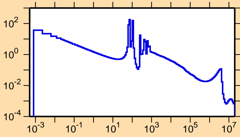
\sigma vs. E for ^{117}\text{Pd}(n,\gamma)
