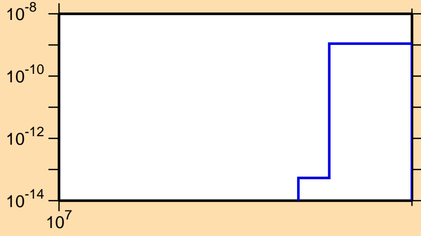
\sigma vs. E for ^{117}\text{Pd}(n,nt)
