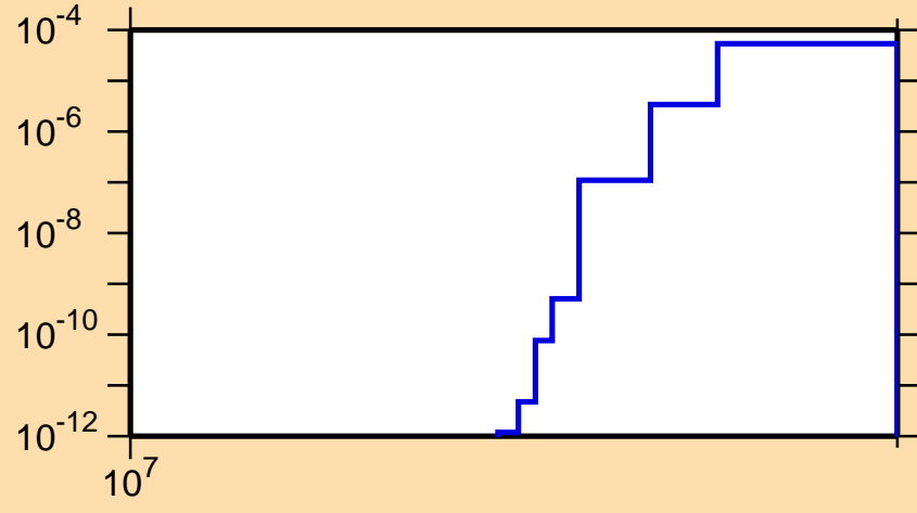
\sigma vs. E for ^{117}\text{Pd}(n,np)
