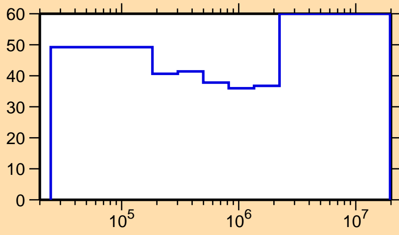
\Delta\sigma/\sigma vs. E for ^{117}\text{Pd}(n,n_1)
