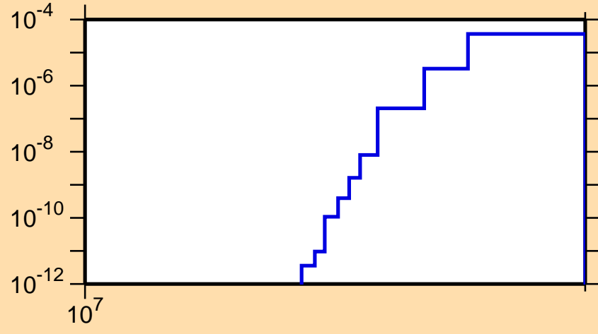
\sigma vs. E for ^{118}\text{Pd}(n,d)
