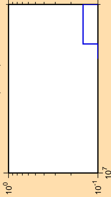
\Delta\sigma/\sigma vs. E for ^{118}\text{Pd}(n,2n\alpha)
