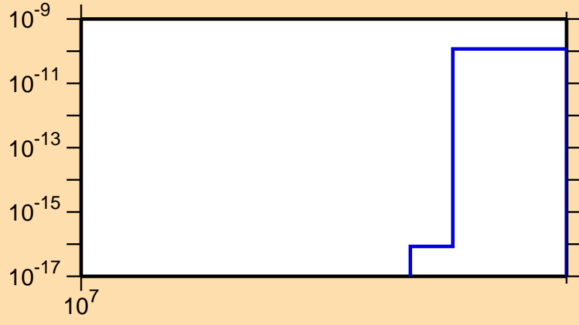
\sigma vs. E for ^{118}\text{Pd}(n,nt)
