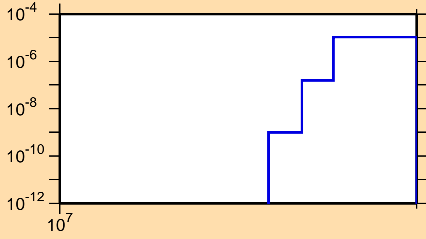
\sigma vs. E for ^{118}\text{Pd}(n,np)
