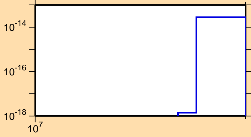
\sigma vs. E for ^{118}\text{Pd}(n,2n\alpha)
