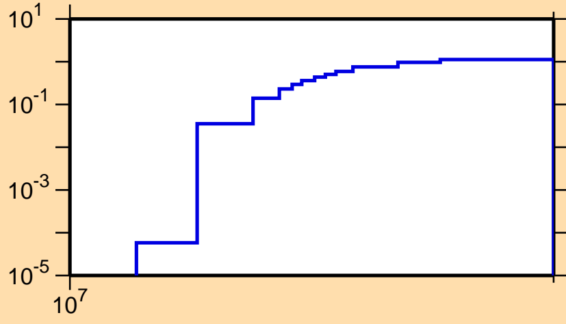
\sigma vs. E for ^{118}\text{Pd}(n,3n)
