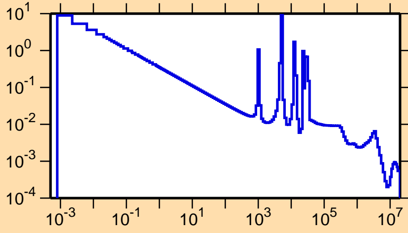
\sigma vs. E for ^{118}\text{Pd}(n,\gamma)
