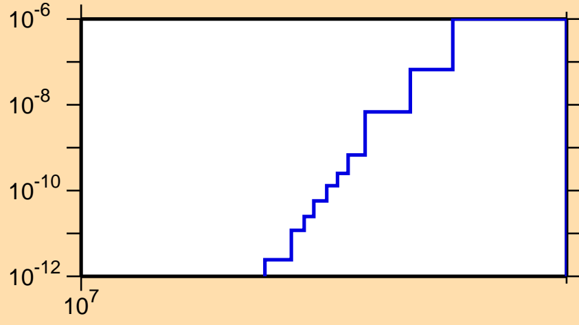
\sigma vs. E for ^{118}\text{Pd}(n,n\alpha)
