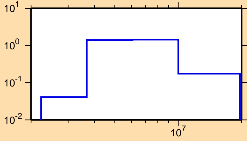
\sigma vs. E for ^{118}\text{Pd}(n,n\text{cont.})
