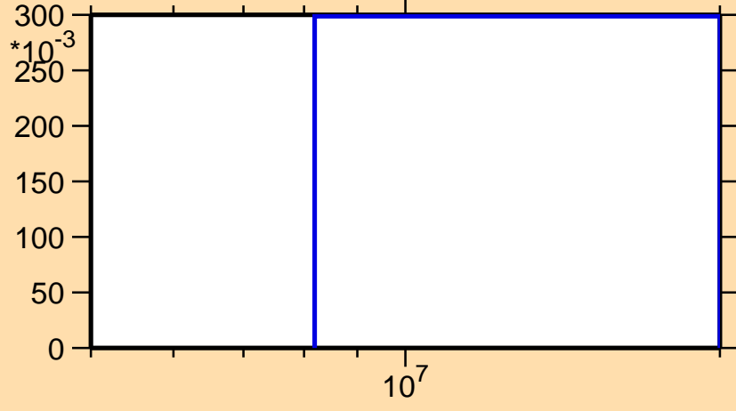
\sigma vs. E for ^{118}\text{Pd}(n,3n)
