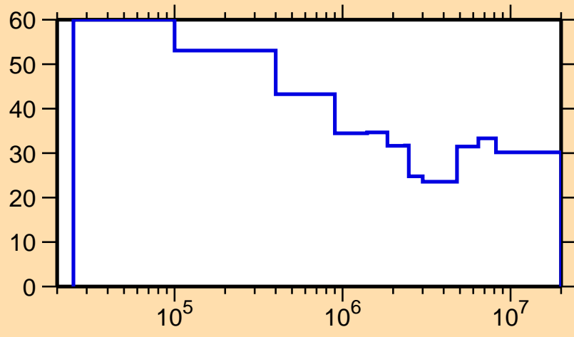
\Delta\sigma/\sigma vs. E for ^{118}\text{Pd}(n,\text{nonel.})
