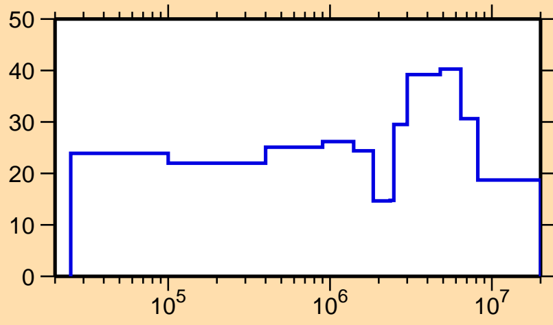
\Delta\sigma/\sigma vs. E for ^{118}\text{Pd}(n,\text{tot.})
