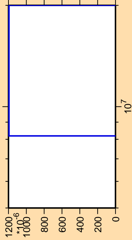
\Delta\sigma/\sigma vs. E for ^{118}\text{Pd}(n,2n\alpha)
