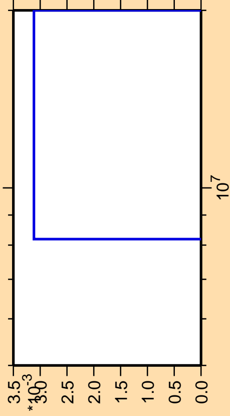
\Delta\sigma/\sigma vs. E for ^{118}\text{Pd}(n,nd)
