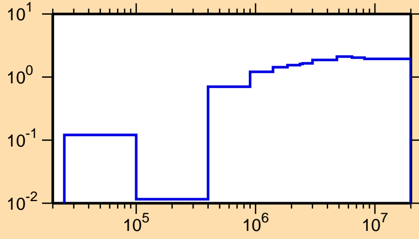
\sigma vs. E for ^{118}\text{Pd}(n,\text{nonel.})
