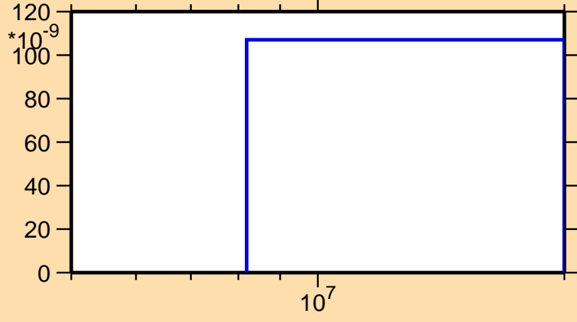
\sigma vs. E for ^{118}\text{Pd}(n,t)
