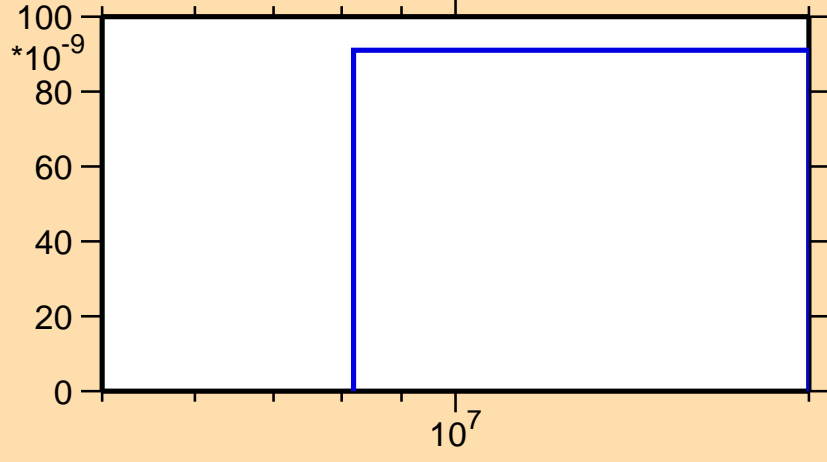
\sigma vs. E for ^{118}\text{Pd}(n,np)
