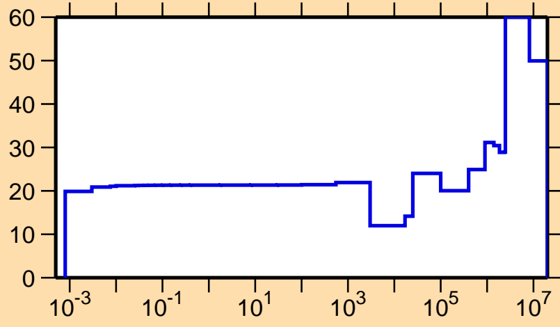
\Delta\sigma/\sigma vs. E for ^{118}\text{Pd}(n,\text{el.})
