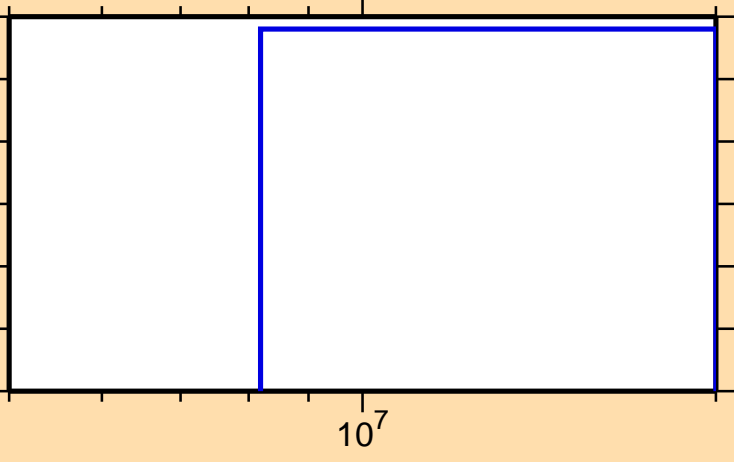
\sigma vs. E for ^{118}\text{Pd}(n,n\alpha)
