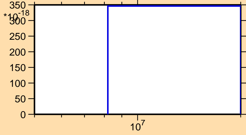
\sigma vs. E for ^{118}\text{Pd}(n,nd)
