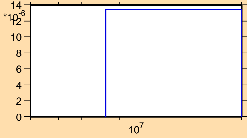
\sigma vs. E for ^{118}\text{Pd}(n,p)
