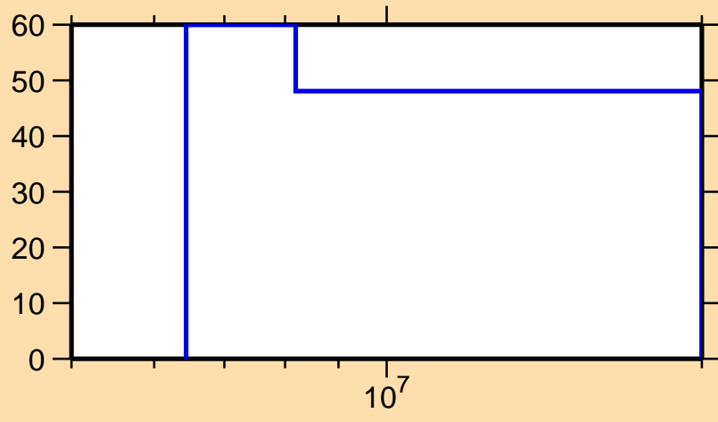
\Delta\sigma/\sigma vs. E for ^{118}\text{Pd}(n,2n)
