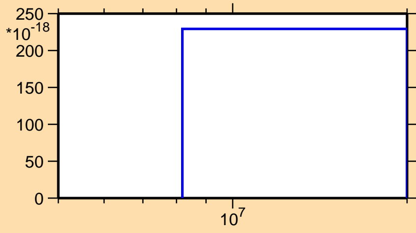
\sigma vs. E for ^{118}\text{Pd}(n,2n\alpha)
