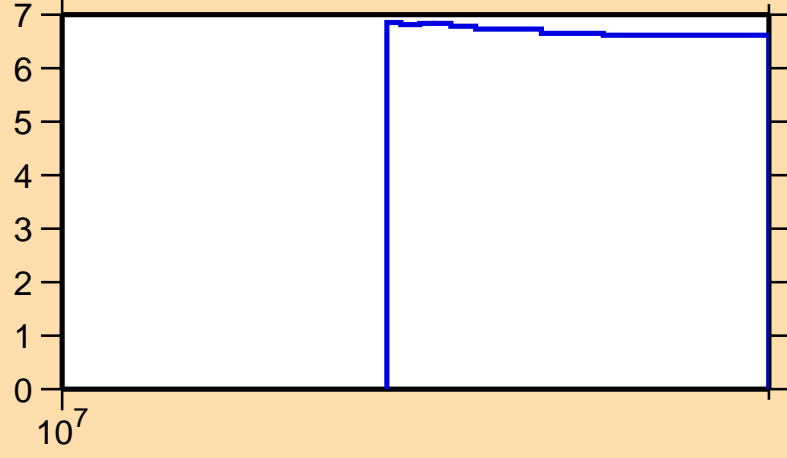
\Delta\sigma/\sigma vs. E for ^{127}\text{Pm}(n,\text{nonel.})
