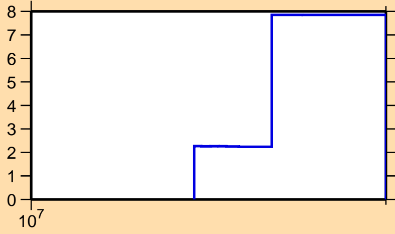
\Delta\sigma/\sigma vs. E for ^{127}\text{Pm}(n,el.)
