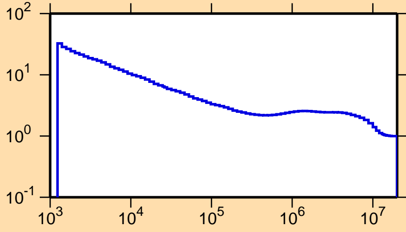
\sigma vs. E for ^{127}\text{Pm}(n,\text{nonel.})
