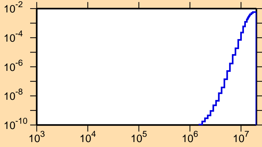
\sigma vs. E for ^{127}\text{Pm}(n,\text{He}3)
