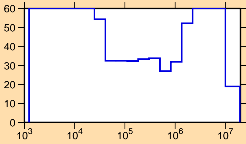
\Delta\sigma/\sigma vs. E for ^{127}\text{Pm}(n,p)
