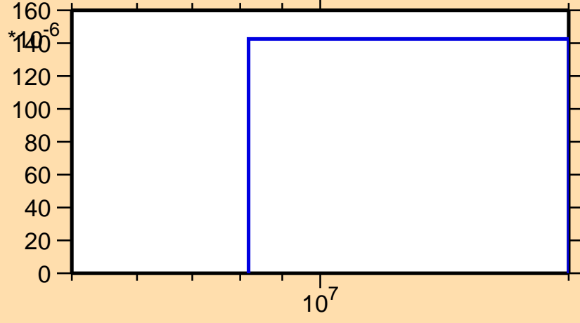
\sigma vs. E for ^{128}\text{Pm}(n,\text{pt})
