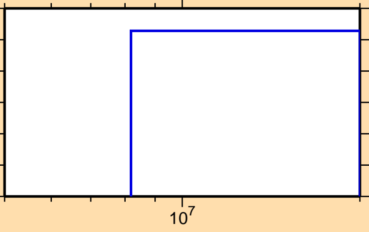
\sigma vs. E for ^{128}\text{Pm} (mt 34)
