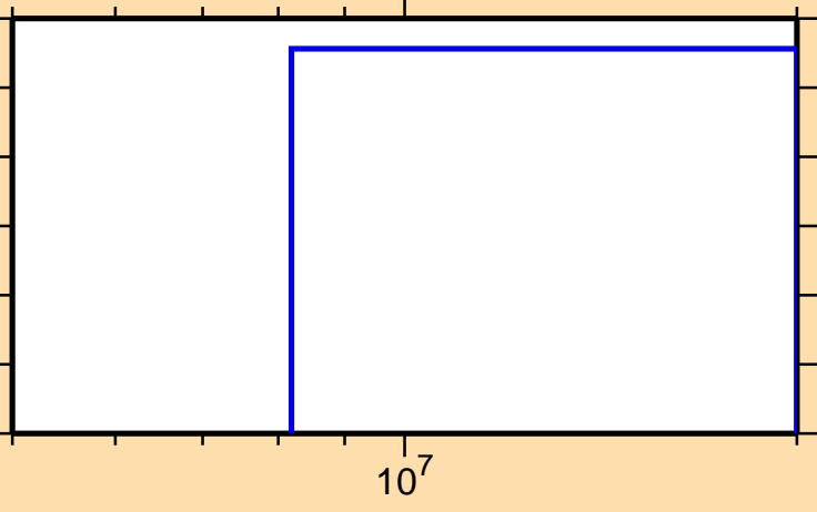
\sigma vs. E for ^{128}\text{Pm}(n,2n)
