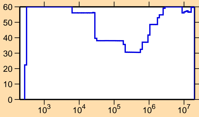
\Delta\sigma/\sigma vs. E for ^{129}\text{Pm}(n,p)
