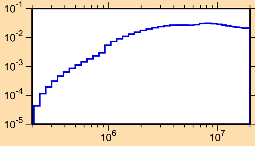
\sigma vs. E for ^{129}\text{Pm}(n,n\text{cont.})
