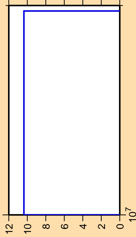
\Delta\sigma/\sigma vs. E for ^{129}\text{Pm}(n,2n\alpha)
