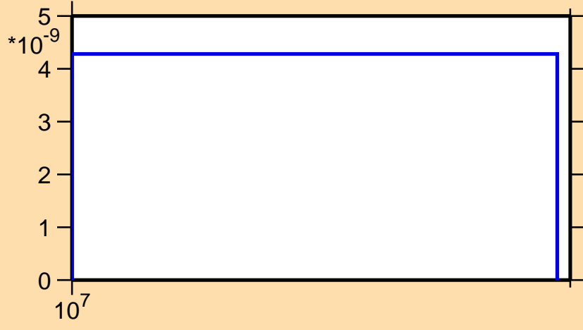
\sigma vs. E for ^{129}\text{Pm}(n,nd)
