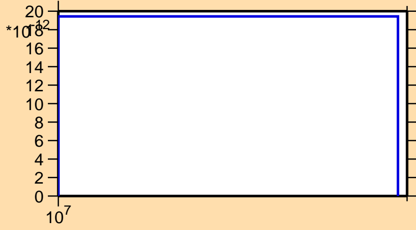
\sigma vs. E for ^{129}\text{Pm} (mt 34)
