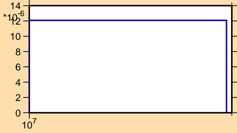
\sigma vs. E for ^{129}\text{Pm}(n,2n)
