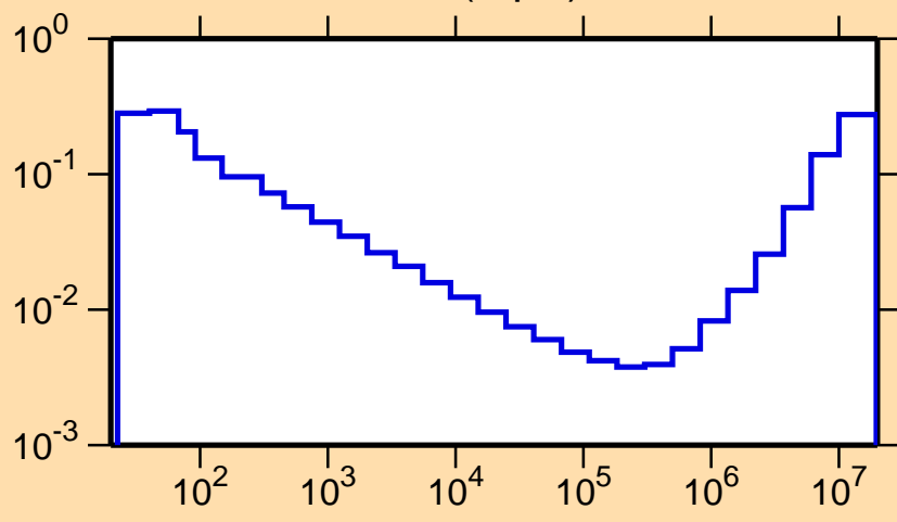
\sigma vs. E for ^{130}\text{Pm}(n,p\alpha)
