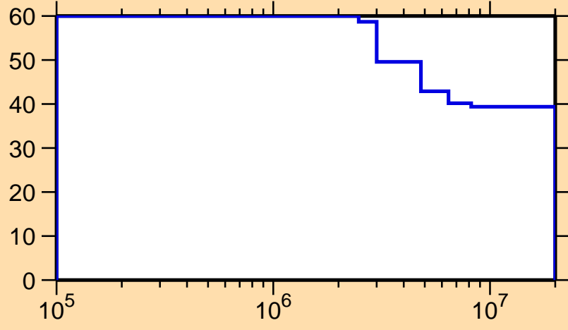
\Delta\sigma/\sigma vs. E for ^{130}\text{Pm}(n,ncont.)
