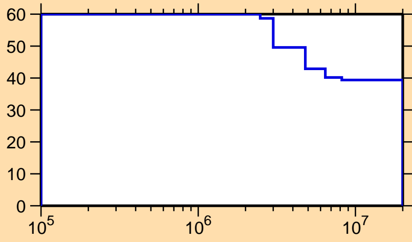
\Delta\sigma/\sigma vs. E for ^{130}\text{Pm}(n,n\text{cont.})
