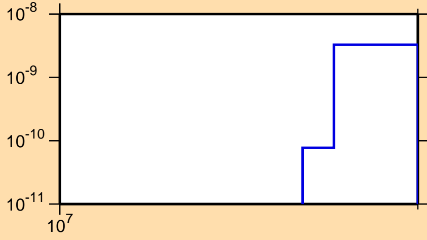
\sigma vs. E for ^{131}\text{Pm}(n,2n\alpha)
