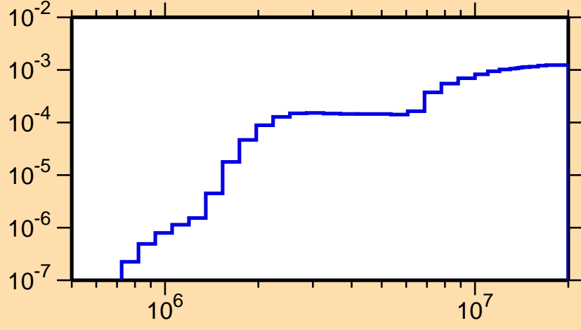
\sigma vs. E for ^{131}\text{Pm}(n,n\text{cont.})
