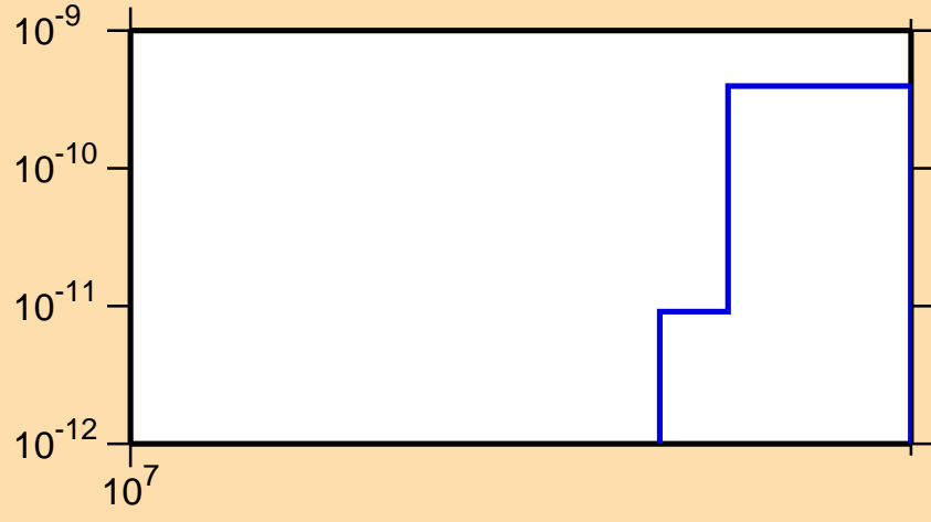
\sigma vs. E for ^{131}\text{Pm} (mt 34)
