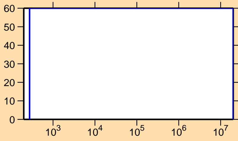
\Delta\sigma/\sigma vs. E for ^{131}\text{Pm}(n,\gamma)
