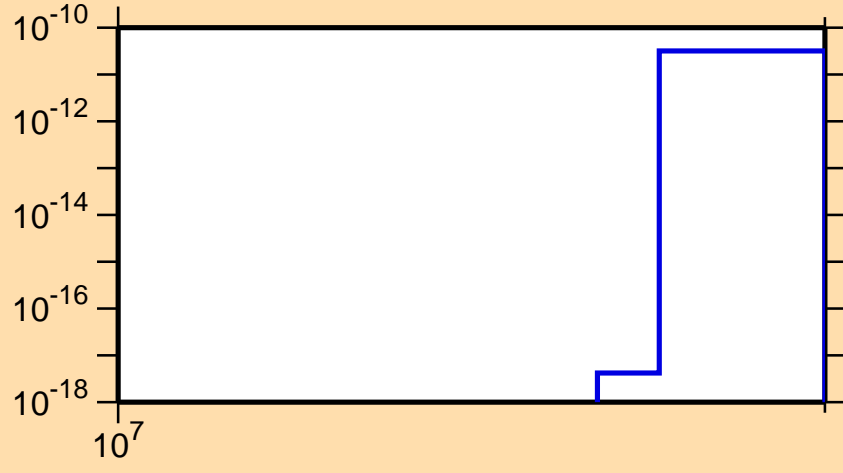
\sigma vs. E for ^{131}\text{Pm}(n,nt)
