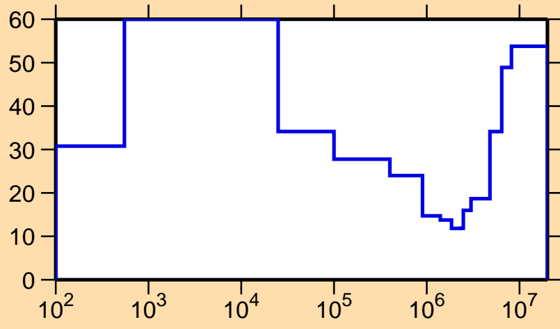
\Delta\sigma/\sigma vs. E for ^{131}\text{Pm}(n,p)
