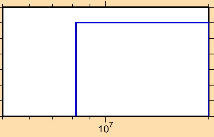
\sigma vs. E for ^{132}\text{Pm}(n,nd)
