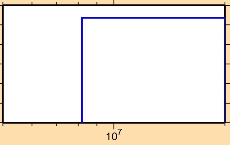
\sigma vs. E for ^{132}\text{Pm} (mt 34)
