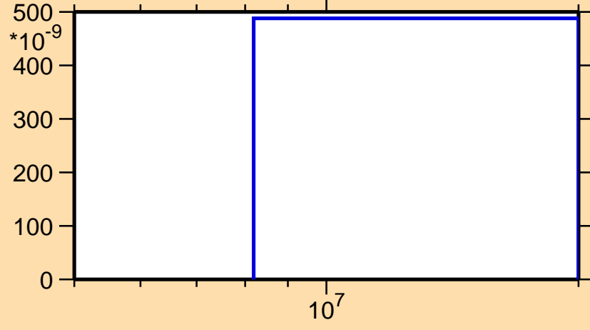
\sigma vs. E for ^{132}\text{Pm}(n,pt)
