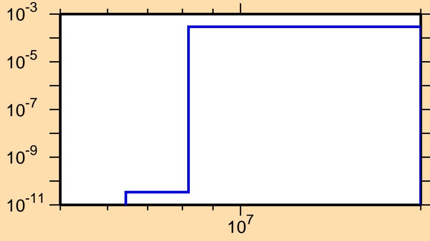
\sigma vs. E for ^{132}\text{Pm} (mt 45)
