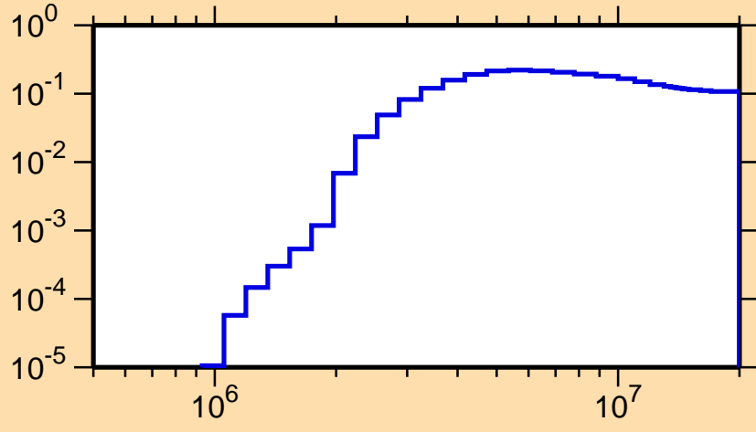
\sigma vs. E for ^{133}\text{Pm}(n,n\text{cont.})
