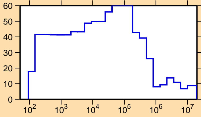
\Delta\sigma/\sigma vs. E for ^{133}\text{Pm}(n,el.)
