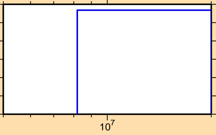
\sigma vs. E for ^{133}\text{Pm}(n,2n)
