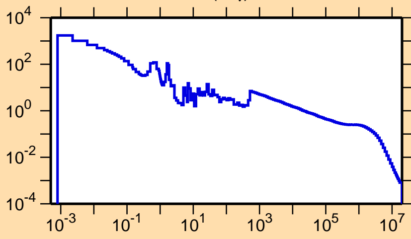
\sigma vs. E for ^{133}\text{Pm}(n,\gamma)
