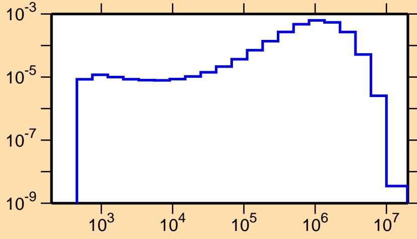
\sigma vs. E for ^{133}\text{Pm}(n,n_1)
