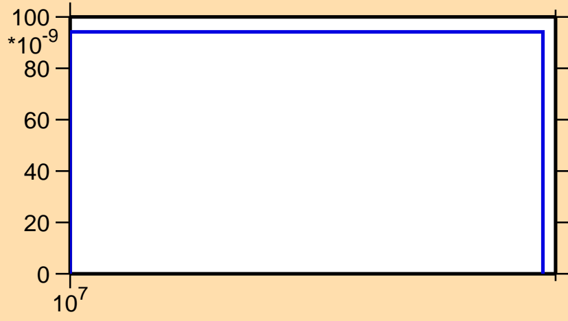
\sigma vs. E for ^{133}\text{Pm}(n,\text{nd})
