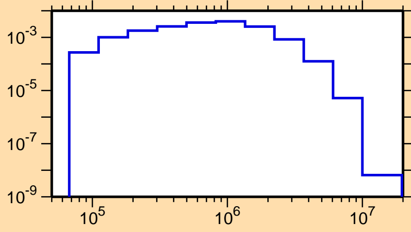
\sigma vs. E for ^{133}\text{Pm}(n,n_4)
