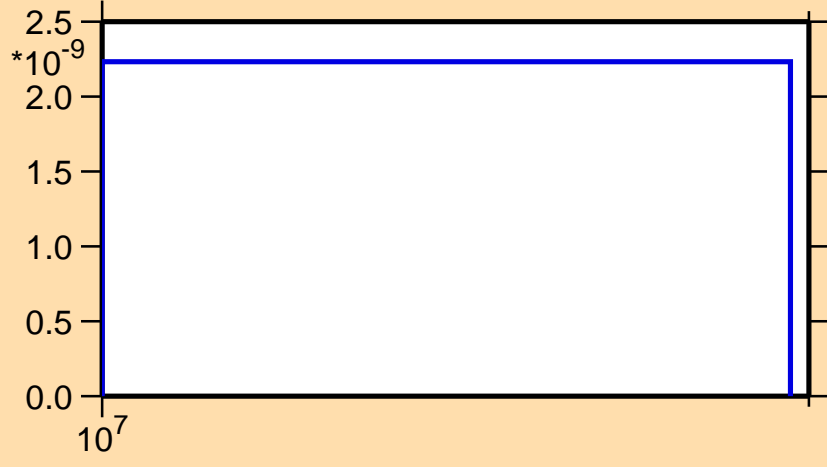
\sigma vs. E for ^{133}\text{Pm}(n,\text{pt})
