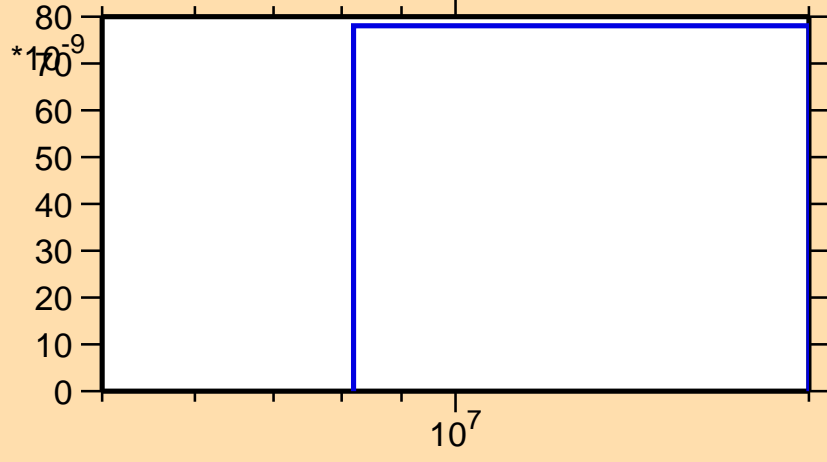
\sigma vs. E for ^{133}\text{Pm}(n,\text{nd})
