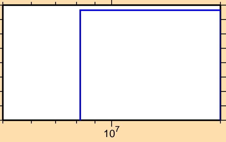
\sigma vs. E for ^{133}\text{Pm}(n,2n\alpha)
