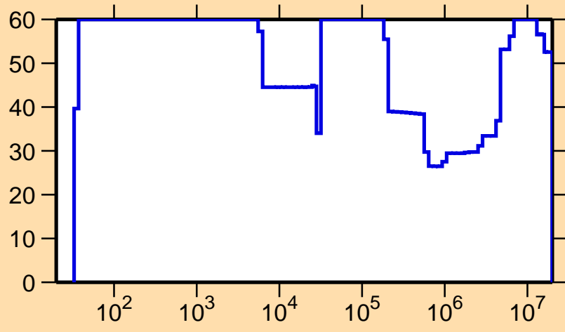
\Delta\sigma/\sigma vs. E for ^{134}\text{Pm}(n,p)
