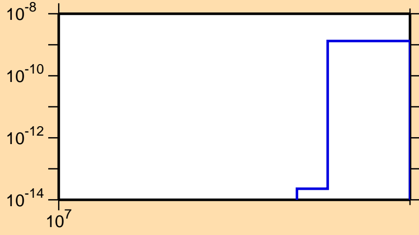
\sigma vs. E for ^{134}\text{Pm}(n,nt)
